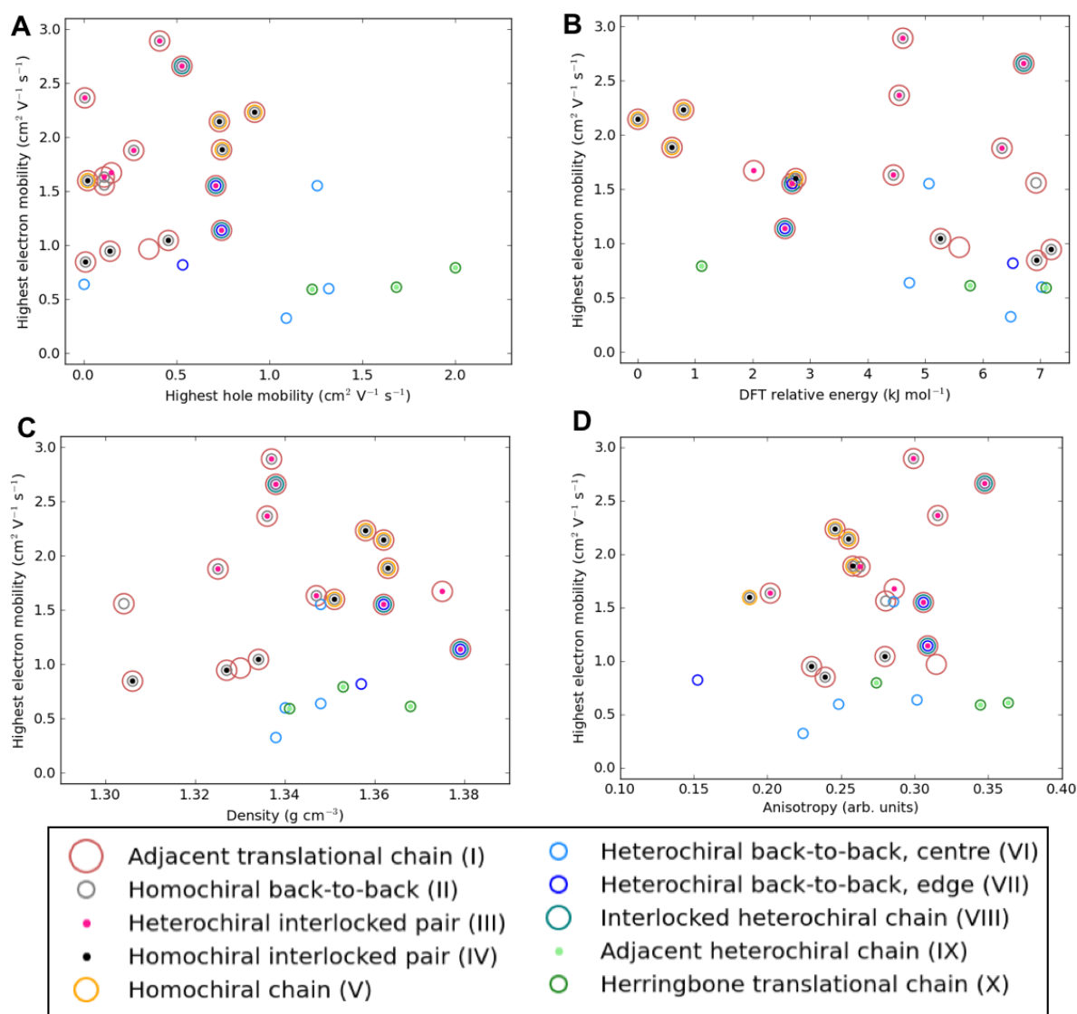
Figure 6: Electron mobility for the energetically low-lying [6]helicene polymorphs compared to (a) hole mobility, (b) DFT relative energy, (c) density and (d) anisotropy of electron mobility. The data points are coloured according to the substructure type. The equivalent plots for hole mobility are in Fig. S10.
