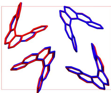
Figure 4: An overlay of the experimental HEXHEL enantiopure structure ( 1 ) viewed down the c axis (red) and the lowest energy computed [6]helicene crystal structure (blue), as relaxed with the B86bPBE-XDM method.
