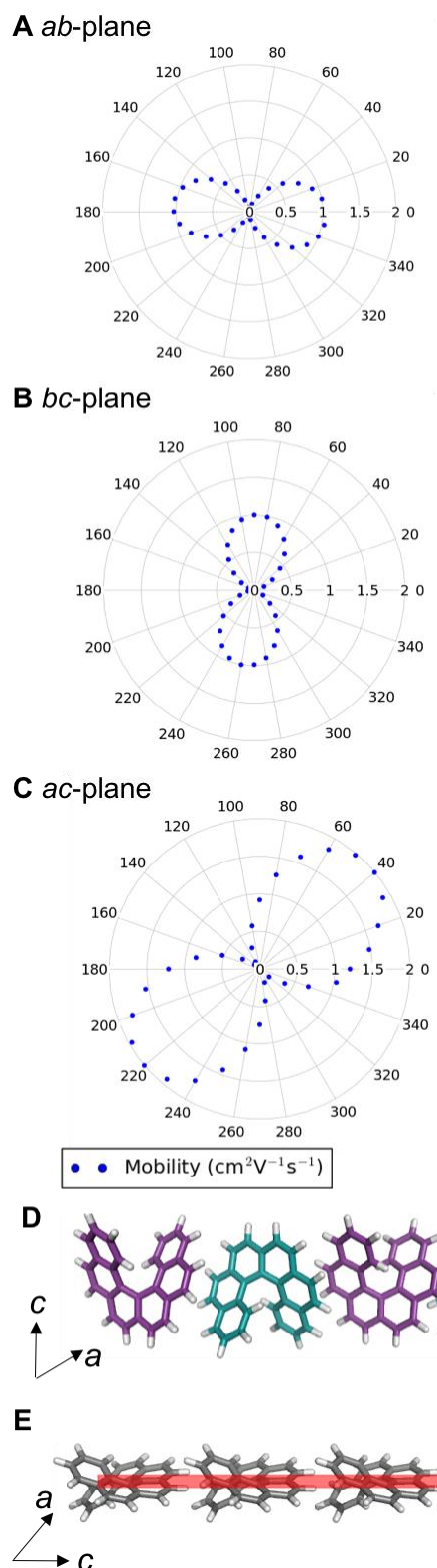
Figure 7: Angular dependent hole mobility for structure 4 in the (a) ab -, (b) bc - and (c) ac - planes; (d) the adjacent heterochiral chain (substructure type IX ) with hole mobility of 0.01 \text{ cm}^2 \text{ V}^{-1} \text{ s}^{-1} (e) the herringbone translational homochiral chain (substructure type X ) with hole mobility of 2.0 \text{ cm}^2 \text{ V}^{-1} \text{ s}^{-1} . The red arrow shows the highest hole mobility direction for structure 4 .
