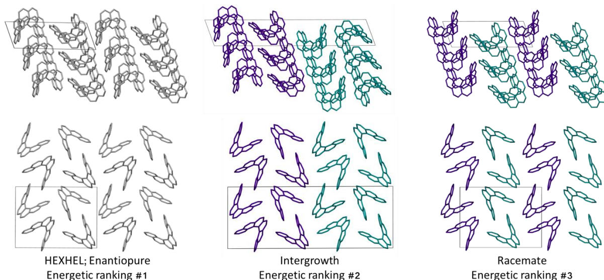
Figure 2: A comparison of the three lowest energy computed [6]helicene structures, each shown in two perpendicular views. In the enantiopure structure, all molecules are grey, in the intergrowth and racemate structures, the left-handed molecule is shown in cyan and the right-handed in purple. The unit cells are shown with a black box; Across all structures in the top row, chains of helicenes with translational symmetry run vertically on the page, while on the bottom row, chains of alternating interlocked and “back-to-back” helicene pairs run vertically on the page.
