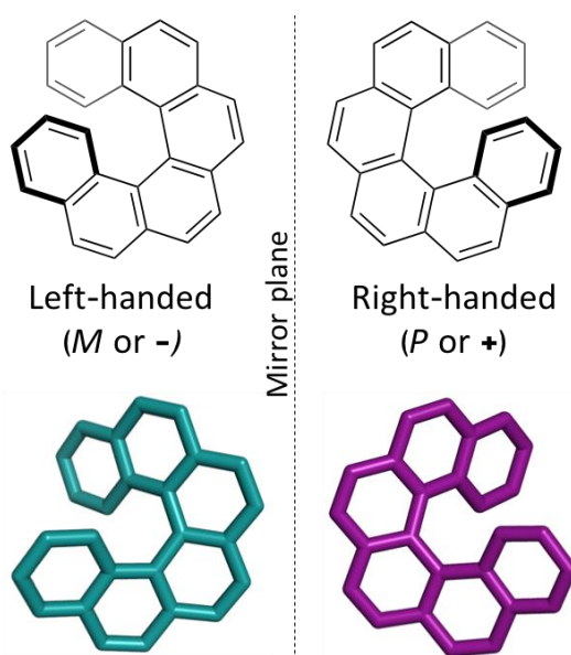
Figure 1: The two enantiomers of the chiral [6]helicene molecule, shown in a top-down view (bold bonds indicate bonds projecting towards the viewer).
