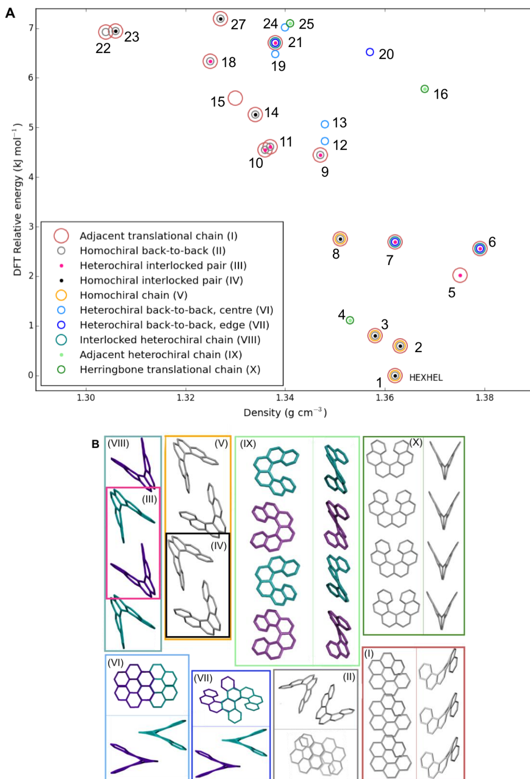
Figure 5: (a) Lattice energy landscape labelled according to which molecular substructures they contain. Substructures are ordered by decreasing frequency. Note, two predicted structures (17 and 26) do not appear on the plot as they contain none of these substructures, for their positions, refer back to Fig. 3; (b) The molecular substructures, with surrounding boxes coloured and labelled as
