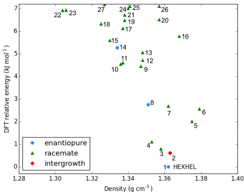
Figure 3: Lattice energy landscape with the B86bPBE-XDM method for the energetically low-lying [6]helicene polymorphs. The structure labelled HEXHEL is the observed enantiopure structure and all structures are numbered according to their final energetic ranking; this numbering is used to refer to the structures throughout the text.
