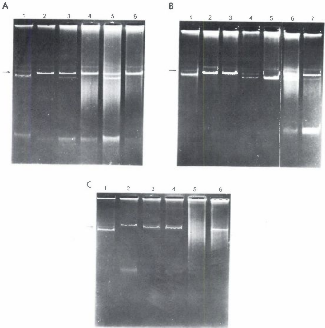
Figure 1. Plasmid profile of plasmid donors, recipients and the resulting transconjugants.
