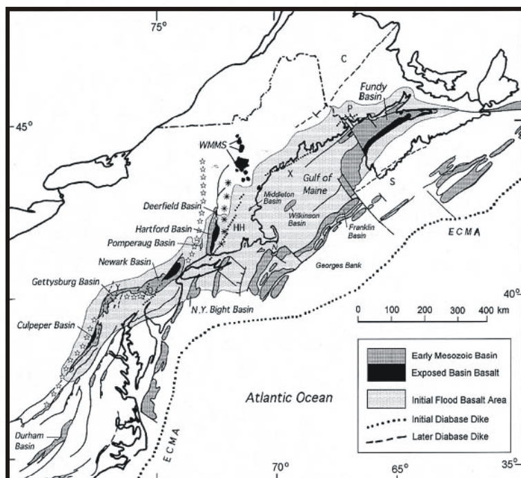
Figure 1. Map showing the extent of the Mesozoic extensional basins in eastern North America showing the Fundy Basin of Maritime Canada at the north end. Note the extent of the East Coast Magnetic Anomaly (ECMA) along the continental margin. From G. McHone web page.
