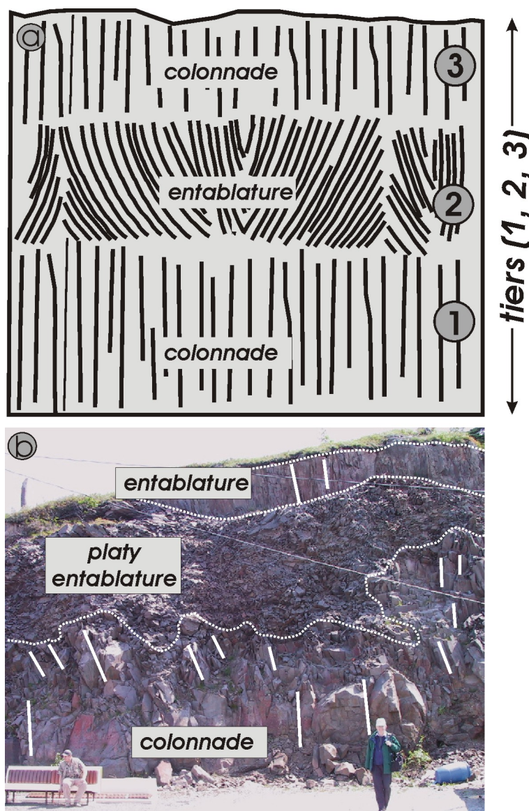
Figure 14. (a) Schematic cross section showing the nature of colonnade and entablature jointing in homogeneous basalt. Note that there is a single flow unit represented here, not three successive flows. (b) Outcrop of UFU basalt at East Ferry, where a similar style of jointing as that shown in Figure 14a is present. The chaotic nature of the entablature reflects differential cooling and relates to the infiltration of water as the basalt was cooling (e.g., Long and Wood, 1986). The orientation of the columns in both the lower and upper colonnade parts of the flow are of variable orientation, also consistent with differential cooling due to the influx of water.
