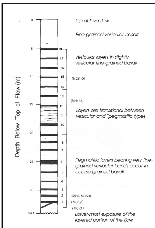
Figure 21. Stratigraphy of the upper 34 m of the thick, layered flow at McKay Head (right column. Numbering on layers (1-18) is schematic. The column marked "Time" gives estimates of the number of years it took the upper crust, growing downward, to reach various levels in the flow. Diagram and information modified from Greenough et al., (1989a) and Greenough and Dostal (1992b).
