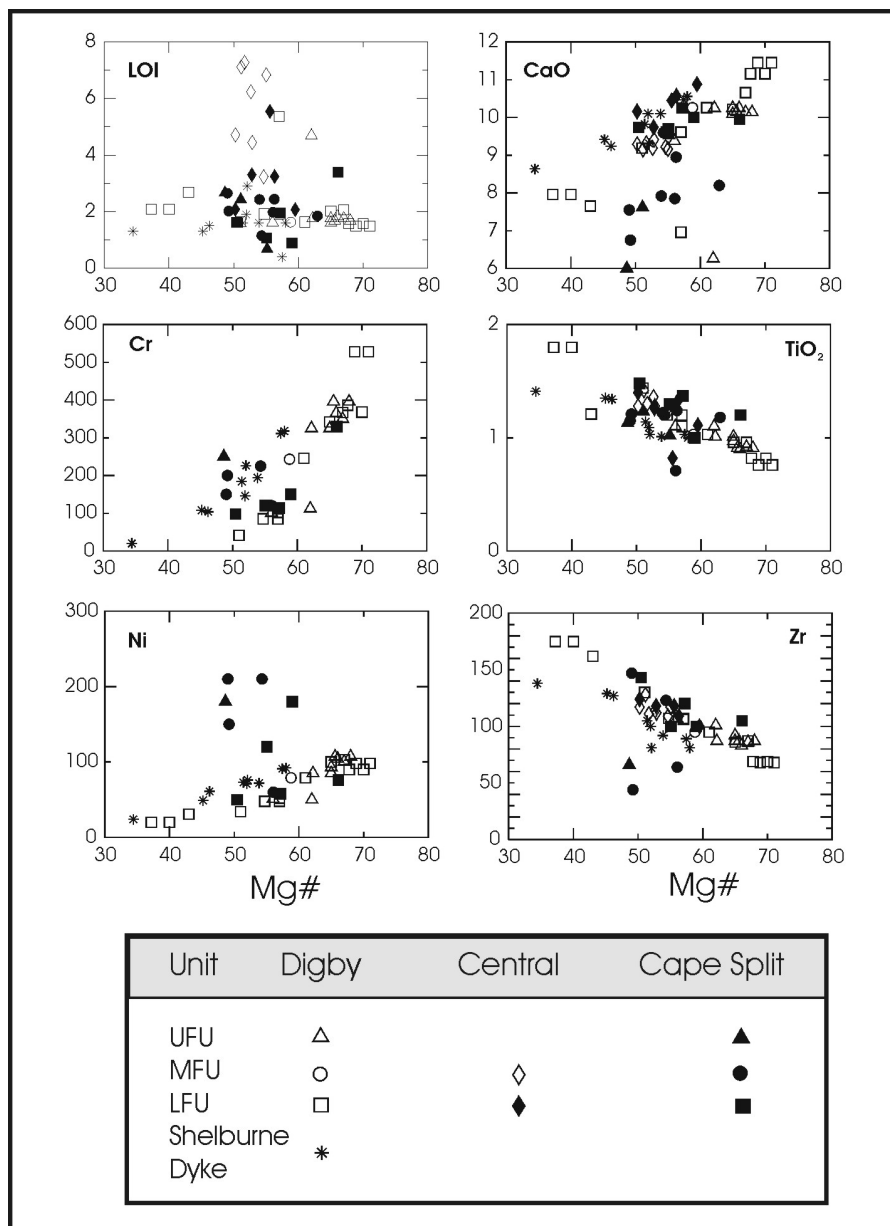
Figure 15. Binary plots of chemical data (wt. % and ppm) for the NMB and the Shelburne dyke with data subdivided into the flow unit (LFU, MFU, UFU) and geographical setting. Note that only data on the southern side of the Bay of Fundy have been used. Mg# is magnesium number (atomic Mg/(Mg+Fe)). Sources of data are from Sinha (1970), Wark and Clark (1980), Papezik et al. (1988) and Dostal and Durning (1998). Note that for the Sinha (1970) data set we have
