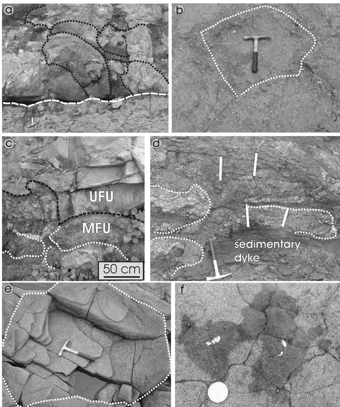
Figure 35. Photographs of outcrops in Sweeney Point area. (a) Breakout lobes (outlined by dashed black lines) on the surface of a sheet lobe, as marked by the dashed white line. Outcrop along beach northeast of parking area at Stop 2. (b) Columnar jointing, colonnade type, in the core zone of a sheet lobe near previous outcrop photo. Note the presence of disseminated amygdules in this part of the flow. Note the large column outlined by the dashed white line. (c) Flow lobes in top of a sheet lobe of the MFU that is overlain by the basal part of the UFU (contact marked by dashed black line). Outcrop near the promontory where UFU outcrops and
