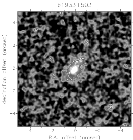
Figure 2. HST WFPC2 F814W ( I -band) image, showing the same region as above, also smoothed to 0.31 arcsec resolution.
