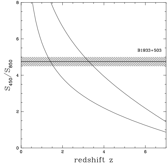
Figure 6. 450 \mu\text{m} to 850 \mu\text{m} flux ratio for different models. The two solid lines span a range of reasonable emissivities and dust temperatures.
