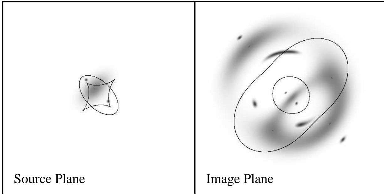
Figure 4. The result of our lens modelling for one particular example of a dusty disc. The left panel represents the source plane, while the right panel is the (observed) image plane. The solid lines denote caustics in the source plane and critical lines in the image plane. Each panel is 1.4 arcsec on a side, and is oriented to align with fig. 1 of Sykes et al. (1998). Darker shading represents both the shallow spectrum (compact source) and shallow spectrum (extended ‘lobes’) radio emission, while lighter grey shows a model of the far-infrared and sub-mm emission from a possible dusty torus. The resulting image configuration can be compared to the observed system.
