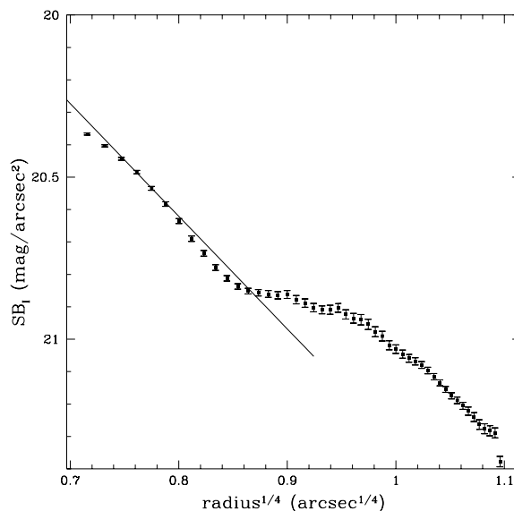
Figure 3. Surface brightness profiles of the CFHT/AOB K -band (top) and HST I -band (bottom) images, smoothed with a 0.31 arcsec boxcar filter, and with an r^{1/4} law fit to the central regions.
