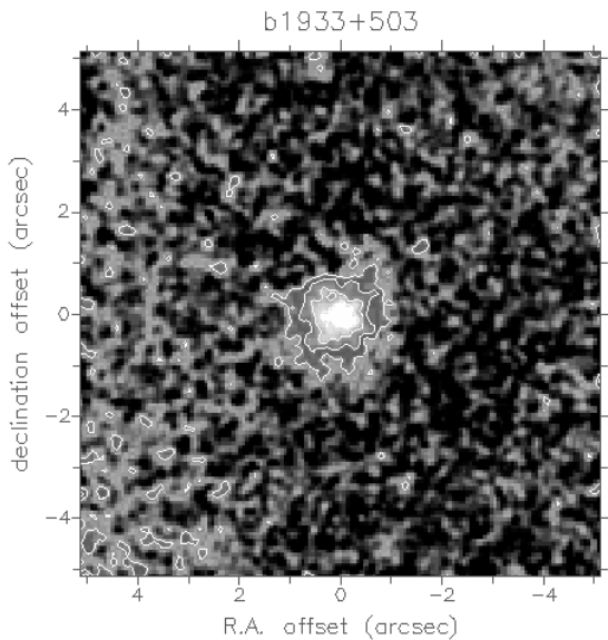
Figure 1. CFHT K -band adaptive optics image of the 10 arcsec \times 10 arcsec field surrounding B 1933, smoothed with a 0.31 arcsec boxcar filter (corresponding to the resolution). There is no indication of a central point source.
