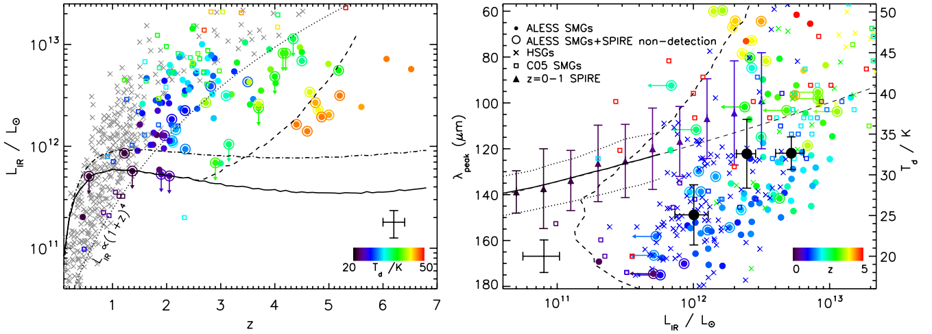
Figure 7. Left: the IR luminosity as a function of photometric redshift for the ALESS SMGs, colour coded by characteristic dust temperature. The dotted line denotes luminosity evolution according to L_{\text{IR}} \propto (1+z)^4 . We also include several selection functions: (i) selection of an S_{870 \mu\text{m}} > 2 \text{ mJy} SMG for a dust SED with characteristic dust temperature of T_d = 32 \text{ K} (solid line); (ii) selection of an S_{870 \mu\text{m}} > 2 \text{ mJy} SMG for a dust SED with characteristic dust temperature that evolves with luminosity and redshift (dot-dashed line) and (iii) S_{870 \mu\text{m}} > 2 \text{ mJy} SMGs which are likely to be detected in at least two SPIRE bands (dashed line). Right: the relation between the characteristic dust temperature (which closely corresponds to the approximate peak wavelength of the dust SED, \lambda_{\text{peak}} ) versus IR luminosity ( L_{\text{IR}} ) for the ALESS SMGs, colour coded by photometric redshifts. To facilitate a useful comparison with other surveys, the characteristic dust temperatures shown here are derived using the grey-body fits to the far-IR photometry at the photometric redshift of each SMG. The dashed line denotes the approximate selection limits for an 870 \mu\text{m} selected sample with S_{870 \mu\text{m}} > 2 \text{ mJy} which are then detected in at least two SPIRE bands. We also plot the (local) 60 \mu\text{m} IRAS L_{\text{IR}} - T_d correlation from Chapman et al. (2003b) (solid line, with 1\sigma dispersion shown by the dotted line; see also Chapin, Hughes & Aretxaga 2009) and also the z = 0-1 SPIRE-selected LIRGs and ULIRGs (Symeonidis et al. 2013). In both panels, we also include recent measurements for SMGs from Magnelli et al. (2012a) which are partly based on the Chapman et al. (2005) (CO5) survey and Herschel star-forming Galaxies (HSGs) from (Casey et al. 2012). In both panels, we also show a representative error bar for our ALESS measurements. The large, solid points in the right-hand panel show the median temperature (and bootstrap error) of ALESS SMGs in bins of far-IR luminosity, showing that the high-redshift SMGs have cooler temperatures ( \Delta T = 3-5 \text{ K} , or equivalently, their dust SEDs peak at longer wavelengths) at fixed luminosity than comparably luminous galaxies at z = 0 , which is likely due to the more extended star formation in these systems.
