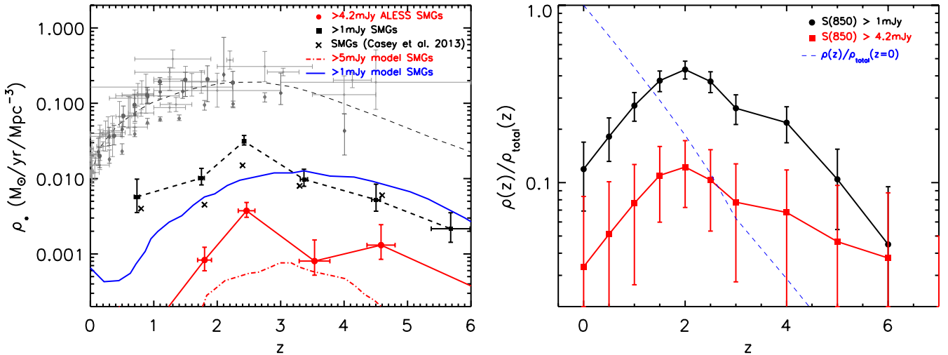
Figure 9. Left: the contribution of SMGs to the comoving cosmic star formation density as a function of redshift. Since the original LESS survey had flux density limits of S_{870\mu\text{m}} = 4.2\text{ mJy} , we only include ALESS SMGs brighter this limit, but then extrapolate to all SMGs brighter than S_{870\mu\text{m}} = 1\text{ mJy} using the 850 \mu\text{m} counts (Coppin et al. 2006). This plot shows that the SMG activity peaks at z \sim 2 – similar to that found by previous studies of star-forming galaxies and the peak activity of quasi-stellar objects (Hopkins, Richards & Hernquist 2007). The contribution from the bright SMGs to the total SFRD also peaks at z \sim 2 where they are responsible for \sim 1\text{--}2 per cent of the Hopkins & Beacom (2006) SFRD, although extrapolating to the faintest SMGs, \sim 1\text{ mJy} suggests SMGs contribute up to 20 per cent of the total SFRD at this epoch. Right: fraction of stellar mass in SMGs ( S_{870\mu\text{m}} > 4.2\text{ mJy} ) compared to the total stellar mass density as a function of redshift. The global stellar mass densities as a function of redshift are taken from Marchesini et al. (2010). This figure shows that at z \gtrsim 2\text{--}3 , the bright SMGs ( S_{870\mu\text{m}} > 4.2\text{ mJy} ) contribute \sim 15 per cent of the total stellar mass budget at that epoch, and make up 3–4 per cent of the present day stellar mass density. Integrating to fainter luminosities, SMGs with 870 \mu\text{m} fluxes brighter than S_{870\mu\text{m}} > 1\text{ mJy} are predicted to contribute \sim 30\text{--}40 per cent of the stellar mass density at z \sim 2 .
