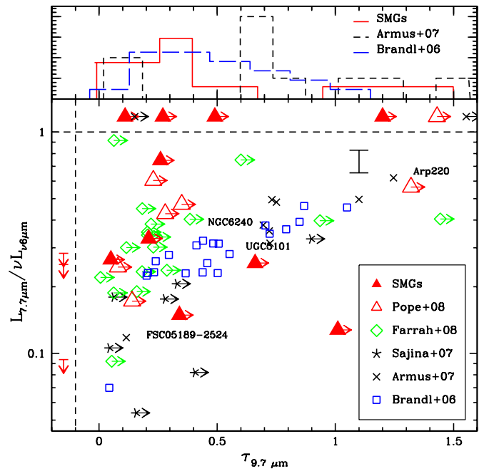
Figure 7. Plot of the 7.7 \mu\text{m} PAH luminosity relative to the 6\text{-}\mu\text{m} continuum luminosity as a function of silicate optical depth. We include optical depth measurements only for those SMGs that provide sufficient wavelength coverage for reasonable continuum estimates: 10 SMGs from our sample and seven SMGs from Pope et al. (2008). Optical depths for local nuclear starbursts (Brandl et al. 2006), local ULIRGs (Armus et al. 2007) and high-redshift 24 \mu\text{m} -selected sources (Sajina et al. 2007; Farrah et al. 2008) are also shown for comparison. Accurate measurements of optical depths require careful determination of the unobscured continuum. We thus quote the values for high-redshift sources displaying low S/N continuum detection at \lambda = 9.7 \mu\text{m} as lower limits. Optical depths measurements for objects for which we do not have continuum measurements at S_{6 \mu\text{m}} are plotted at \text{Log}(L_{7.7}/L_6) > 1 ; upper limits for \text{Log}(L_{7.7}/L_6) in SMGs with no \tau_{9.7 \mu\text{m}} measurements are shown at \tau_{9.7 \mu\text{m}} < -0.1 . The error bar displays the median uncertainty in the SMG PAH-to-continuum ratios. The histogram at the top shows the distributions for SMGs and the two low-redshift samples. SMGs display \tau_{9.7 \mu\text{m}} limits lower than local ULIRGs and the most obscured starbursts, but have proportionally stronger 7.7 \mu\text{m} PAH emission.
