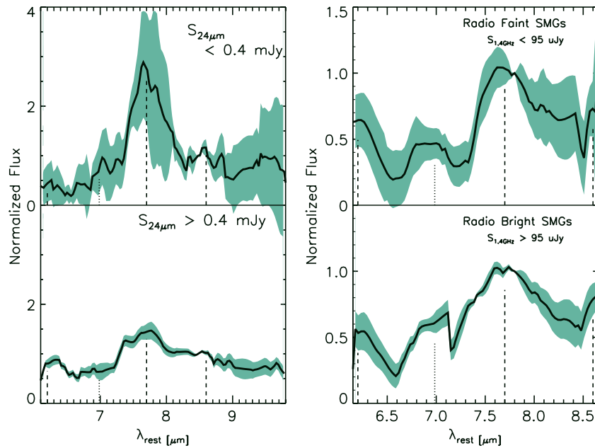
Figure 8. Left: the composite spectra of the seven 24\ \mu\text{m} -bright SMGs within the L_{8\ \mu\text{m}} -complete sample (bottom) and of the seven 24\ \mu\text{m} -faint SMGs (top). Right: composite spectra of the five radio-bright SMGs within the L_{1.4\ \text{GHz}} -complete sample (bottom) and of the five radio-faint SMGs (top). We normalize the spectra of the individual SMGs that comprise the radio composites at \lambda = 7.8\ \mu\text{m} . The 24\ \mu\text{m} -faint composite is significantly more PAH-dominated than the 24\ \mu\text{m} -bright composite, while the latter displays a stronger continuum. In the case of the radio composites, the radio-bright sample appears to display a broader 7.7\ \mu\text{m} PAH feature over a slightly more prominent continuum. However, characterization of the radio-composite spectra does not reveal any significant difference within our measurement uncertainties (see Table 3).
