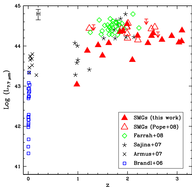
Figure 5. PAH luminosities for the 7.7\ \mu\text{m} feature as a function of redshift for the SMGs in our sample. In addition, we plot the SMGs from Pope et al. (2008). For comparison, we also plot aperture-corrected low-redshift nuclear starburst-dominated galaxies (Brandl et al. 2006), local ULIRGs from the IRAS Bright Galaxy Sample (Armus et al. 2006, 2007) and high-redshift mid-IR-selected sources (Sajina et al. 2007; Farrah et al. 2008). We see that SMGs are among the most PAH-luminous objects in the universe, with PAH features up to 1000\times and 10\times more luminous than local starbursts and ULIRGs, respectively. Considering that PAH emission is associated with strong star-forming activity, this suggests that the SMG population comprises some of the most vigorous star formation events ever observed. See Section 4.2 for discussion.
