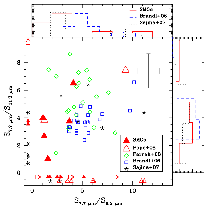
Figure 6. Distribution of 7.7/6.2 and 7.7/11.3 PAH ratios within the SMG population. Objects for which we have only measurable 7.7/6.2 PAH ratios are plotted at S_{7.7}/S_{11.3} < 0 and those for which we only have 7.7/11.3 measurements are plotted at S_{7.7}/S_{6.2} < 0 . We also include PAH ratios measured for a sample of low-redshift nuclear starbursts (Brandl et al. 2006), and high-redshift mid-IR-selected sources (Sajina et al. 2007; Farrah et al. 2008). SMGs share similar 7.7/11.3 PAH ratios with these populations, but their distribution in 7.7/6.2 PAH ratios is skewed toward values that are in general lower than that of low-redshift starbursts. We suggest that this difference in 7.7/6.2 PAH ratio may arise due to a difference in extinction (see Sections 4.2 and 5.2 for discussion).
