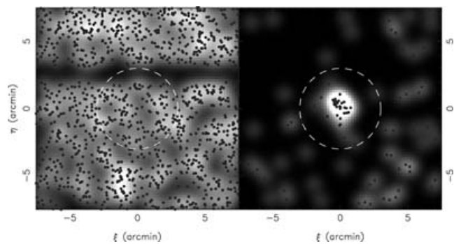
Figure 6. Distribution of galaxies (left-hand panel) and stars (right-hand panel) in the region around And XIII. White pixels represent high-density regions. The maps are highly dissimilar (two-dimensional K–S probability < 10^4 ) showing it is improbable that And XIII is in fact a misidentified background galaxy cluster. The void at \eta \sim 2.5 arcmin is due to a gap between CCDs in the observations.
