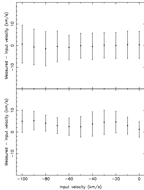
Figure 3. The systematic error in velocity as determined from the analysis of synthetic spectra, using sky residuals as determined from the data. The error bars represent the uncertainty in the velocity determination. The top panel uses Poisson sampling of the median sky, whereas the lower panel uses the median skies from separate CCDs. The overall results show no substantial velocity systematics in the range of -100 \rightarrow 0 \text{ km s}^{-1} , and are typically \sim 1 \text{ km s}^{-1} in the upper panel, increasing to \sim 4\text{--}5 \text{ km s}^{-1} in the lower panel.
