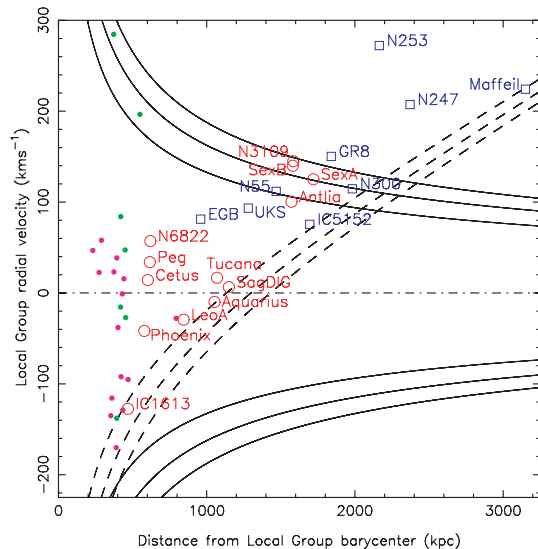
Figure 7. The barycentric Local Group distance versus the Local Group radial velocity for various dwarfs in the local universe. Here, the open circles (red online) are other candidate isolated Local Group dwarf galaxies, the open squares (blue online) represent galaxies belonging to other nearby groups, while the dark-grey and light-grey solid circles (magenta and green online, respectively) represent dwarf galaxies which are satellites of M31 and the Milky Way, respectively.
