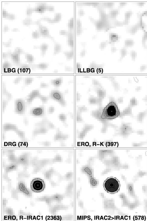
FIG. 2.—Stacked S/N images ( 33'' \times 33'' ) at the positions of the galaxies described in § 4: conventional and IR-luminous LBGs ( top panels ), DRGs and R - K_s > 5.3 EROs ( middle panels ), and IRAC-selected EROs and MIPS-selected galaxies with S_{4.5\mu\text{m}} > S_{3.6\mu\text{m}} ( bottom panels ). Areas of high noise and galaxies detected individually ( \geq 5\sigma ) were excluded. Contours are plotted at S/N levels of -3, 3, 4, \dots, 10, 20, \dots, 100 , and the gray scale is identical in each case. The number of stacked sources from each population is shown in parentheses. The detection of the IRAC-selected ERO population is so significant that we see secondary structure: the image resembles the dirty beam since none of the individually undetected sources in the ensemble that makes up the stacked image have been CLEANed.
