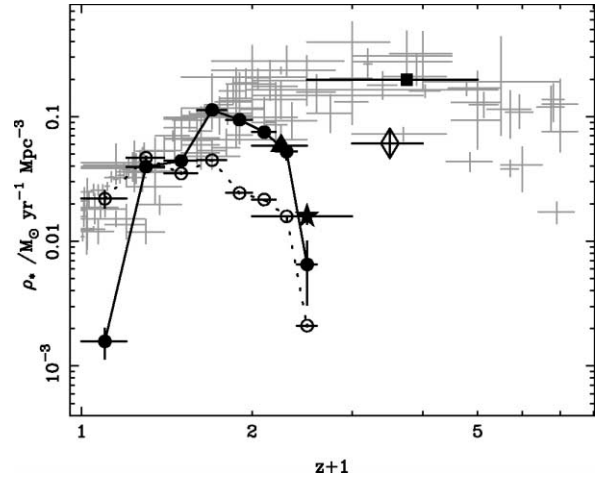
FIG. 1.—Radio-based estimates of SFR density ( \rho_* ) for a number of independent and overlapping galaxy populations selected via magnitude and color criteria: UV-selected galaxies ( open and filled circles for UV- and radio-based SFRs, joined by dotted and solid lines ), R - K_s > 5.3 EROs ( filled triangle ), DRGs ( filled star ), ILLBGs ( open diamond ), and 24 \mu\text{m} -selected galaxies ( filled square ). These are conservative estimates—no attempt has been made to correct for accessible volume; contamination by radio-loud AGNs is possible at z \gg 1 (§ 5). The upper envelope of points thus traces the minimum \rho_* as a function of redshift, as demonstrated by the compilation of \rho_* data from Hopkins & Beacom (2006), plotted faintly here. [See the electronic edition of the Journal for a color version of this figure.]
