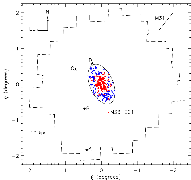
Figure 1. Locations of the new clusters (black stars) are shown in relation to the “high-confidence” clusters in the SM07 catalog (red circles) and the “probable clusters” of ZKH08 (blue circles). The Stokutė et al. (2008) cluster, M33-EC1, is labeled, and an arrow indicates the direction to M31. The solid ellipse indicates the R_{25} isophote and the dashed outline indicates the extent of our INT/WFC survey coverage. The outermost of the new clusters, along with the remote extended cluster of Stokutė et al. (2008), project on the far side of M33 with respect to M31.
