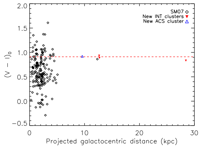
Figure 4. Plot of the extinction-corrected color vs. radius for the cluster population in M33. The dashed line indicates the mean extinction-corrected color of the outer halo GCs in the MW and M31 from Huxor et al. (2009).
