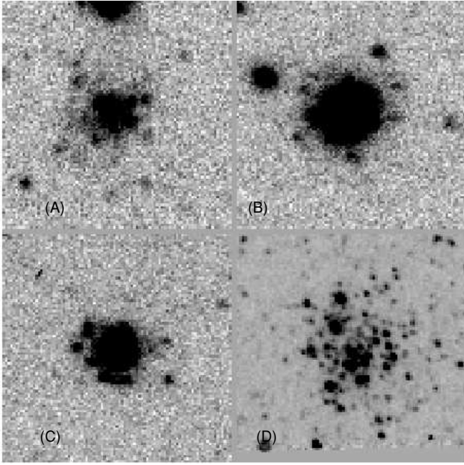
Figure 2. Thumbnails ( i -band) of the outer halo clusters found in the INT-WFC survey (A, B, and C) and in the F606W HST /ACS data (D). The INT images span 30'' \times 30'' while the ACS image spans 7'' \times 7'' . North is up and east is to the left.
