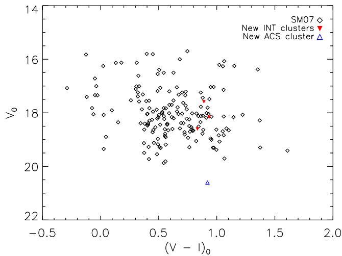
Figure 3. Plot of extinction-corrected color vs. apparent magnitude for the new INT/WFC clusters (inverted triangles), the new ACS cluster (triangle), and the “high-confidence” SM07 sample (open diamonds).
