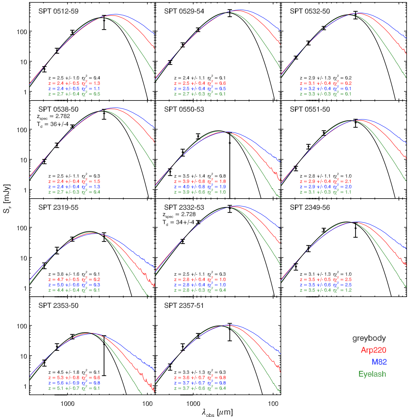
Figure 4. Observed submm/mm SEDs for the 11 sources presented here. The black symbols are SABOCA ( 350 \mu\text{m} ) data, LABOCA ( 870 \mu\text{m} ) data, and SPT photometry ( 1.4 and 2.0 mm). The black curves are modified blackbody fits with fixed spectral index ( \beta = 2.0 ) and T_d = 34 K taken from the median value of the unlensed sample of SMGs. Spectroscopic redshifts break the T_d/(1+z) degeneracy (Blain et al. 2003), and in those cases we quote the best-fit dust temperature. The red, blue, and green curves represent the best-fit SEDs to the data based on the Arp 220, M82, and Eyelash SED templates, respectively (see Section 3.3), where the absolute scaling and the redshift have been allowed to vary (the latter is given in each panel). The graybody fit in black is the simplest curve that fits the data. Without additional photometry shortward of 350 \mu\text{m} , it is difficult to discriminate between different SED templates such as Arp 220 or M82.
