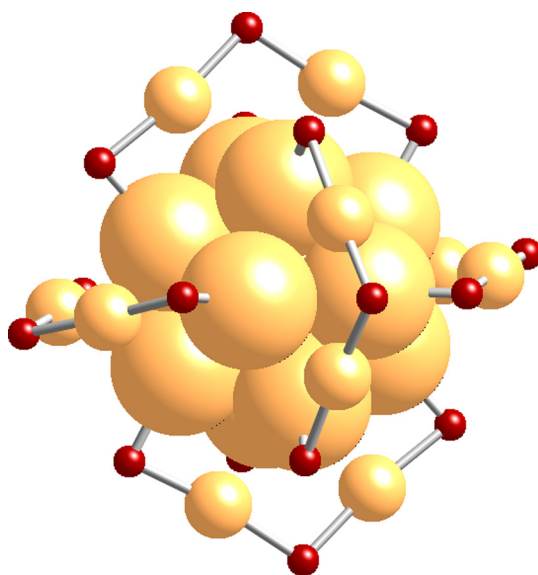
Fig. 1 A model of the Au 25 NC with surface staple motif “S-Au-S-Au-S”. Organic capping ligands are omitted for clarity of the Au 25 NC structure.
