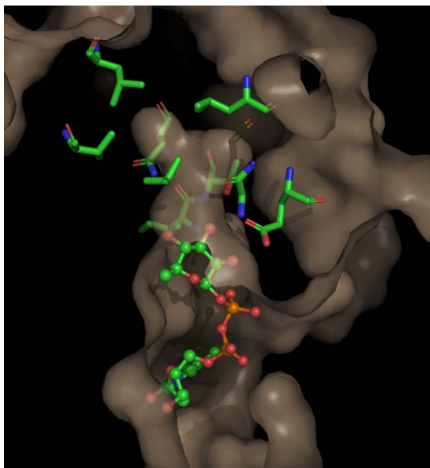
Fig. 2 A cut-away view of the structure of RmlA from Pseudomonas aeruginosa (pdb: 1G3L) showing dTDP- \beta -L-rhamnose (ball-and-stick representation) bound to the solvent accessible enzyme surface. Only residues forming a pocket surrounding the rhamnose moiety are shown for clarity.
