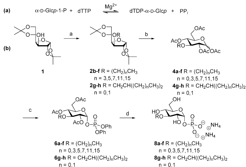
Scheme 1 (a) Physiological reaction catalyzed by \alpha -D-glucopyranosyl-1-phosphate thymidyltransferases, and (b) synthesis of 3-O-alkyl- \alpha -D-glucopyranosyl phosphates: (a) RBr, NaH, DMF, 17–76%; (b) (i) Amberlite 120 H + , 5 : 1 MeOH–H 2 O, 60 °C; (ii) Ac 2 O, py, 32–100%; (c) (i) hydrazine acetate, DMF; (ii) ClPO(OPh) 2 , DMAP, CH 2 Cl 2 , 23–61%; (d) (i) H 2 , PtO 2 , 1 : 1 EtOAc–EtOH; (ii) 2 : 2 : 1 MeOH–H 2 O–NEt 3 , 50 °C; (iii) Amberlite 120 H + , NH 4 OH, 42–100%.
