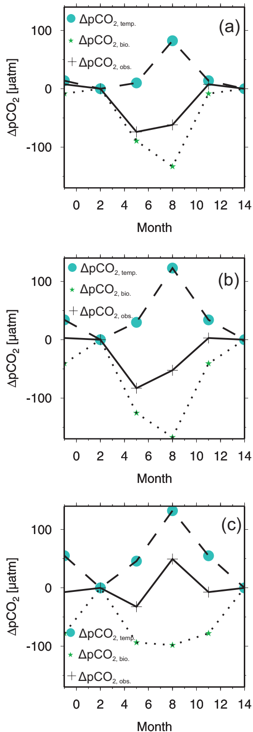
Fig. 4. Biological, temperature and observed \Delta p\text{CO}_2 signals for three different regions of the North Sea: (a) 60^\circ\text{N } 1^\circ\text{E} , (b) 56^\circ\text{N } 1^\circ\text{E} , and (c) 54^\circ\text{N } 3^\circ\text{E} . The data are shown as difference to February.
