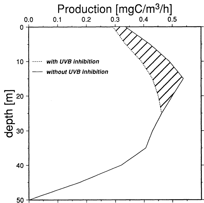
Figure 2. Average values for in situ phytoplankton productivity [ \text{mgCm}^{-3}\text{h}^{-1} ] versus depth[m] within the marginal ice zone of the Bellingshausen Sea in austral spring of 1990. Comparison of productivity inside the ozone hole (stratospheric ozone levels less than 200 Dobson Units, DU) with productivity outside the hole (stratospheric ozone levels greater than 300 DU). Higher UV-B levels (inside the ozone hole) are consistently associated with reduced (left-hand curve) levels of production. Integration of these curves shows that higher UV-B levels within the ozone hole lead to a reduced water column production (6 to 12%). Adapted from Science, 1992, 255:952-959).
