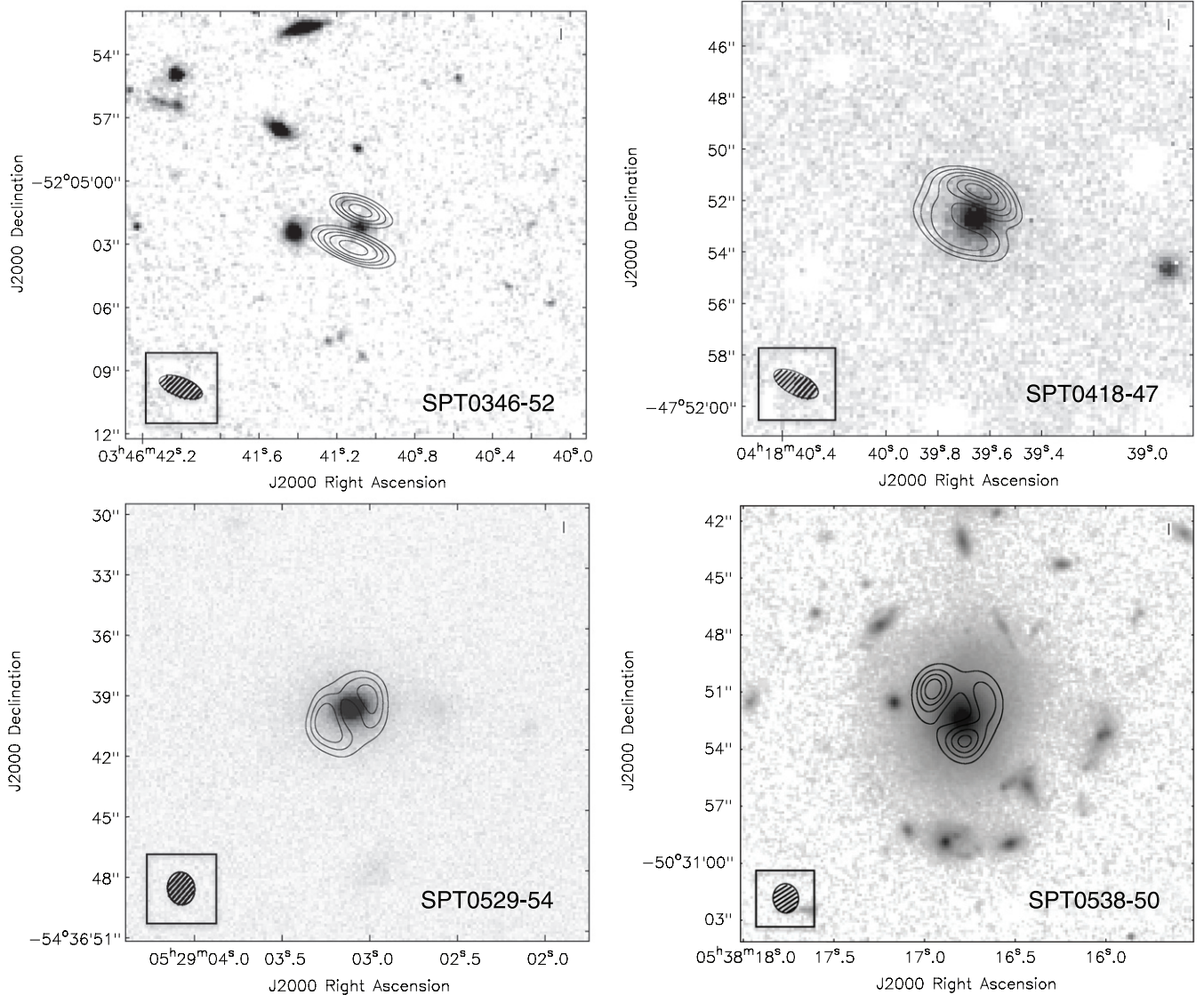
Figure 1. ALMA 350 GHz CLEANed images of the lensed DSGs (contours), on top of NIR imaging of the galaxy field (grayscale) from Hubble Space Telescope , VLT, and SOAR. From left to right, they are SPT0346-52 ( HST ) and SPT0418-47 (VLT) in the top row and SPT0529-54 (SOAR) and SPT0538-50 ( HST ) in the bottom row. The ALMA contours begin at 5\sigma , increasing in steps of 10\sigma in the top left and bottom right images, and 5\sigma in the other two, as in Figure 4. The synthesized beam is shown in the lower left of each image. The HST images are a composite of the F110W and F160W filters, the VLT images are K band from ISAAC, and the SOAR image is K band from OSIRIS.
