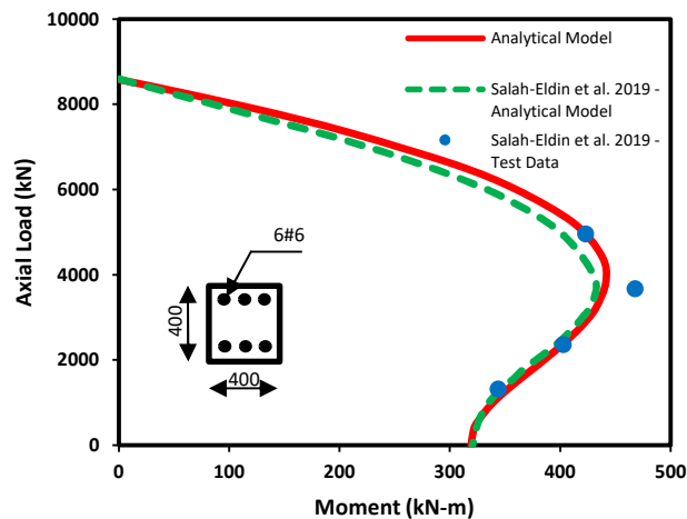
Fig 4. Beam interaction diagram - axial load vs bending moment (Salah-Eldin et al. 2019)
