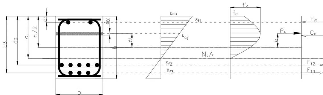
Fig 1. Stress and strain profile of GFRP beam cross-section
