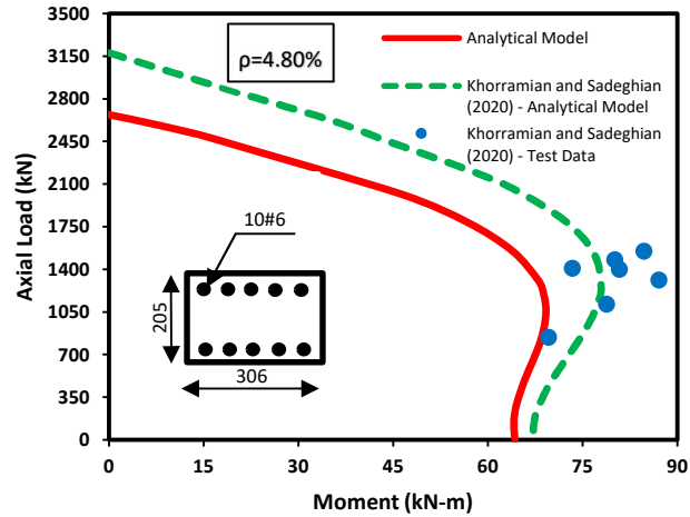
Fig 3. Beam interaction diagram – axial load vs bending moment (Khorramian and Sadeghian 2020)
