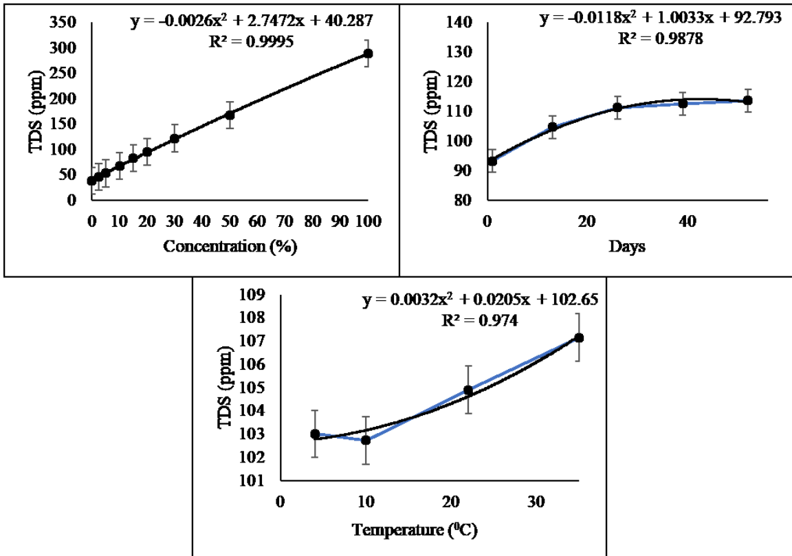
Figure 3.3 Effect of concentration, storage duration and storage temperature on total dissolved solids (TDS) of compost tea.
