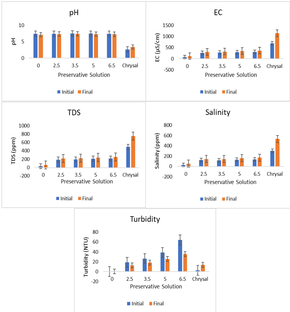
Figure 4.2 Initial (Day 1) and final (Day 11) values of pH, electrical conductivity (EC), turbidity, total dissolved solids (TDS) and salinity of different concentrations of compost tea and Chrysal.
