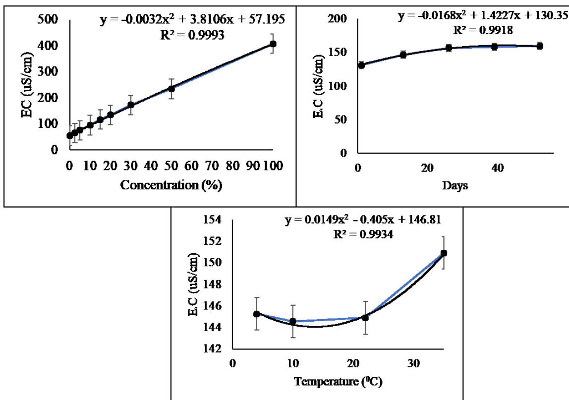
Figure 3.2 Effect of concentration, storage duration and storage temperature on electrical conductivity (E.C) of compost tea.
