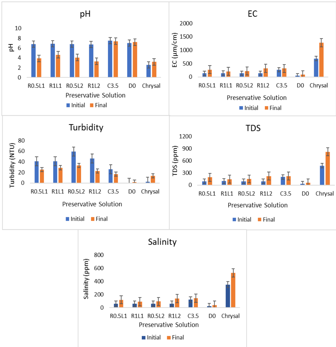
Figure 5.1 Initial (Day 1) and final (Day 11) values of pH, electrical conductivity (EC), turbidity, total dissolved solids (TDS) and salinity of different mixed preservative solutions and the synthetic chemical, Chrysal.
