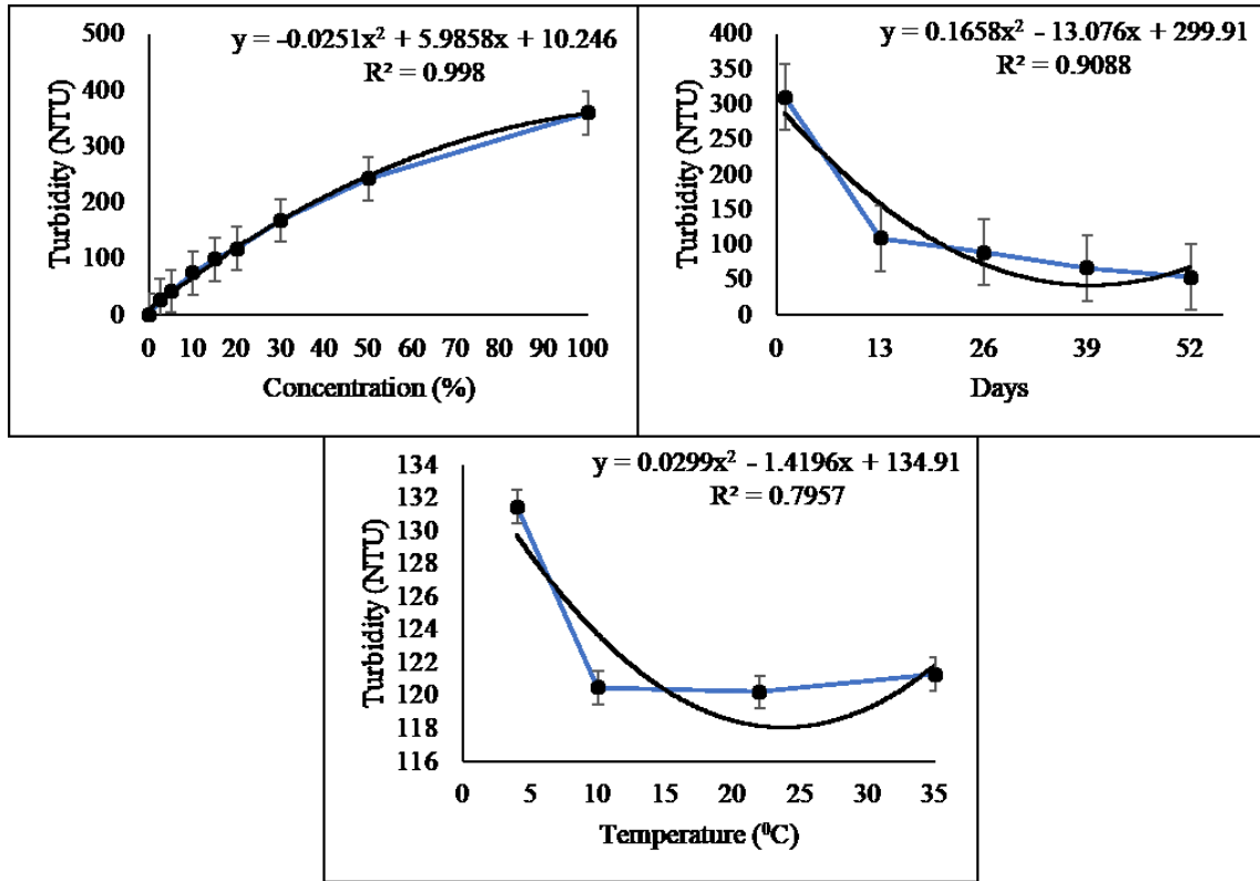
Figure 3.5 Effect of concentration, storage duration and storage temperature on turbidity of compost tea.
