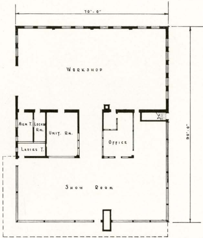
FLOOR PLAN
