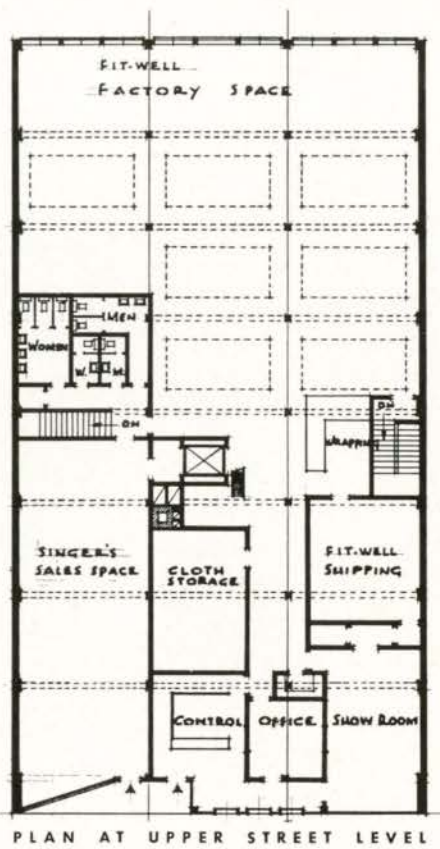
PLAN AT UPPER STREET LEVEL
