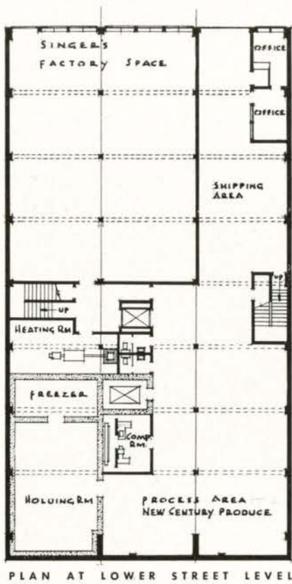
PLAN AT LOWER STREET LEVEL
