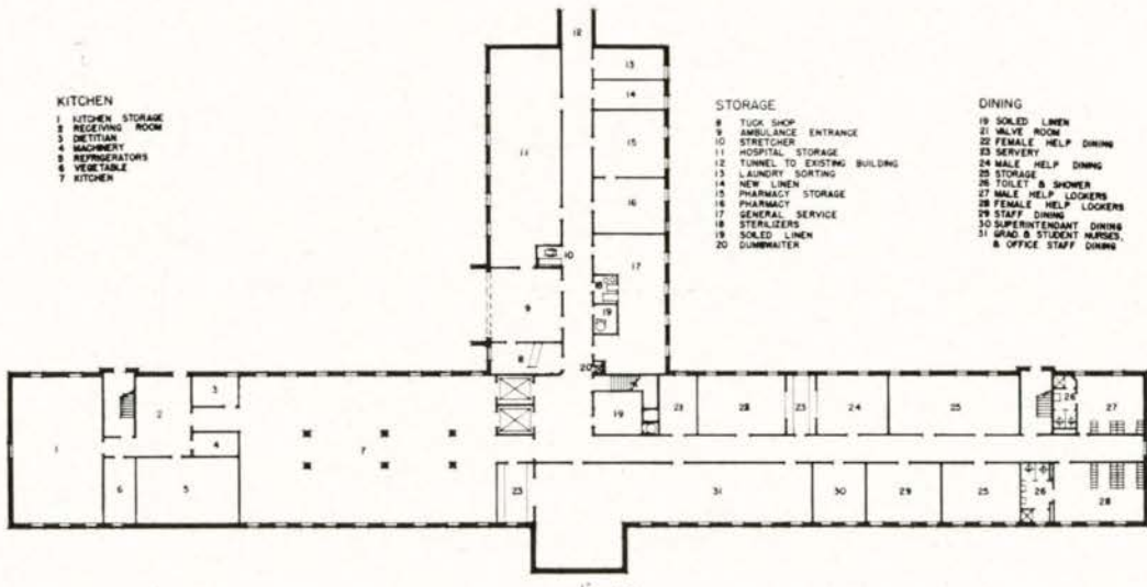
BASEMENT PLAN
