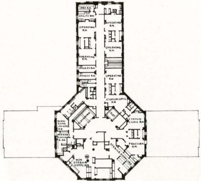
PLAN OF 12th FLOOR
