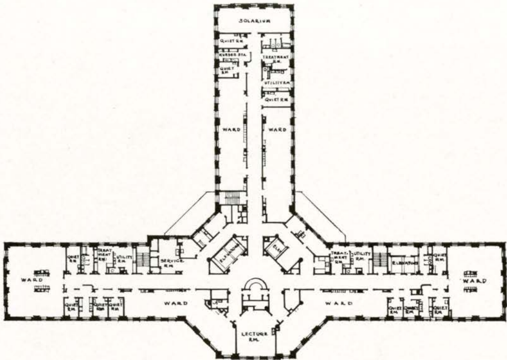
PLAN OF 4th, 5th AND 6th FLOORS
