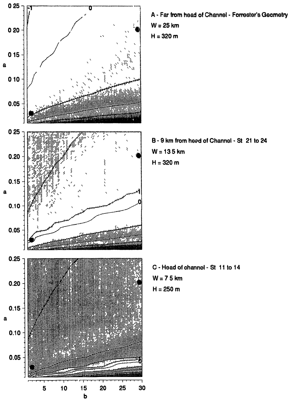
Figure 7.5: Wavenumber k_{21} ( \times 10^4 ) for various a and b values. Negative values found above the zero line—are in fact imaginary (e-folding decay wavenumber). Dots indicate both Forrester's choice for a and b and the alternate choice with second mode node depth of 20 m. A- W = 25 \text{ km} and H = 320 \text{ m} , corresponding to the far field geometry of the channel used by Forrester; B- W = 13.5 \text{ km} and H = 320 \text{ m} , corresponding to the channel geometry at stations 21–24; C- W = 7.5 \text{ km} and H = 250 \text{ m} , corresponding to the channel geometry at stations 11–14.
