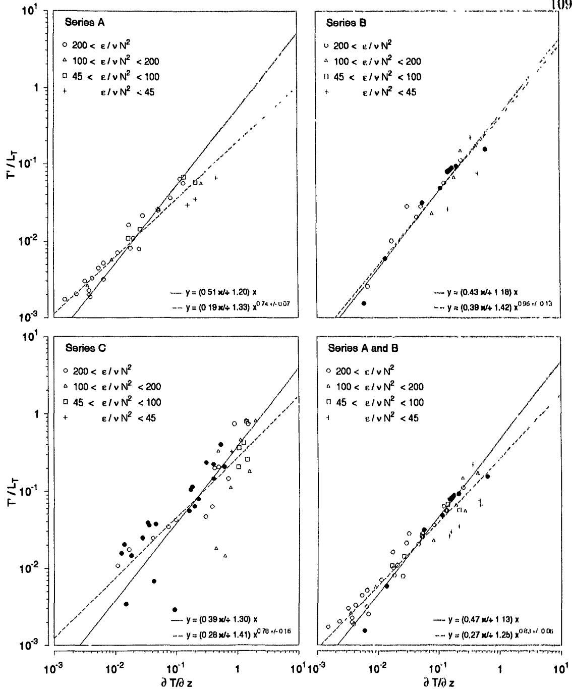
Figure 5.1: Comparison of estimated temperature gradient within overturns \overline{T'^2}^{1/2}/L_T to measured gradient \partial\overline{T}_o/\partial z for two oceanic cases (Series A and B) and a fresh water reservoir (Series C). The gradient \partial\overline{T}/\partial z is evaluated on the re-ordered profile over overturn-containing spans; \overline{T'^2}^{1/2}/L_T is an estimate of the local gradient within the overturns and is found to be lower than \partial\overline{T}_o/\partial z . Data are classified by turbulent intensity \epsilon/\nu N^2 . Open symbols are well resolved; filled symbols are marginally resolved. Regression are on points with \epsilon/\nu N^2 > 200 . Data are from tables in Dillon (1982).
