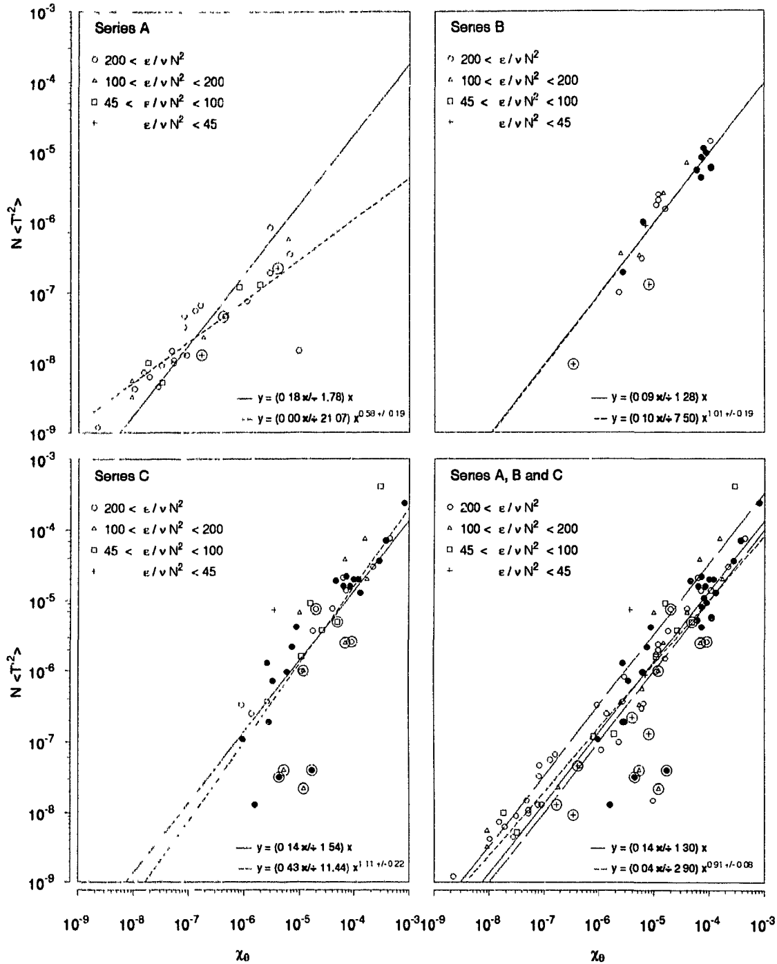
Figure 3.3: Comparison of NT^{r2} vs \chi_0 . The long-dashed lines in the series A, B and C panel are NT^{r2} = 3\chi_0 and NT^{r2} = 10\chi_0 , quoted from Dillon as the range of the scatter. Regressions are on data with \epsilon/\nu N^2 > 200 . Data are coded according to turbulent intensity according to the legend; open symbols are well resolved data, filled symbols are marginally resolved; circled data have (\overline{T}^{1/2}/L_T)/(\partial\overline{T}/\partial z) < 0.2 . Data are from tables in Dillon (1982); both axes are in ^\circ\text{C}^2 \text{ s}^{-1} . This figure corresponds somewhat to Figure 7 in Dillon (1982).
