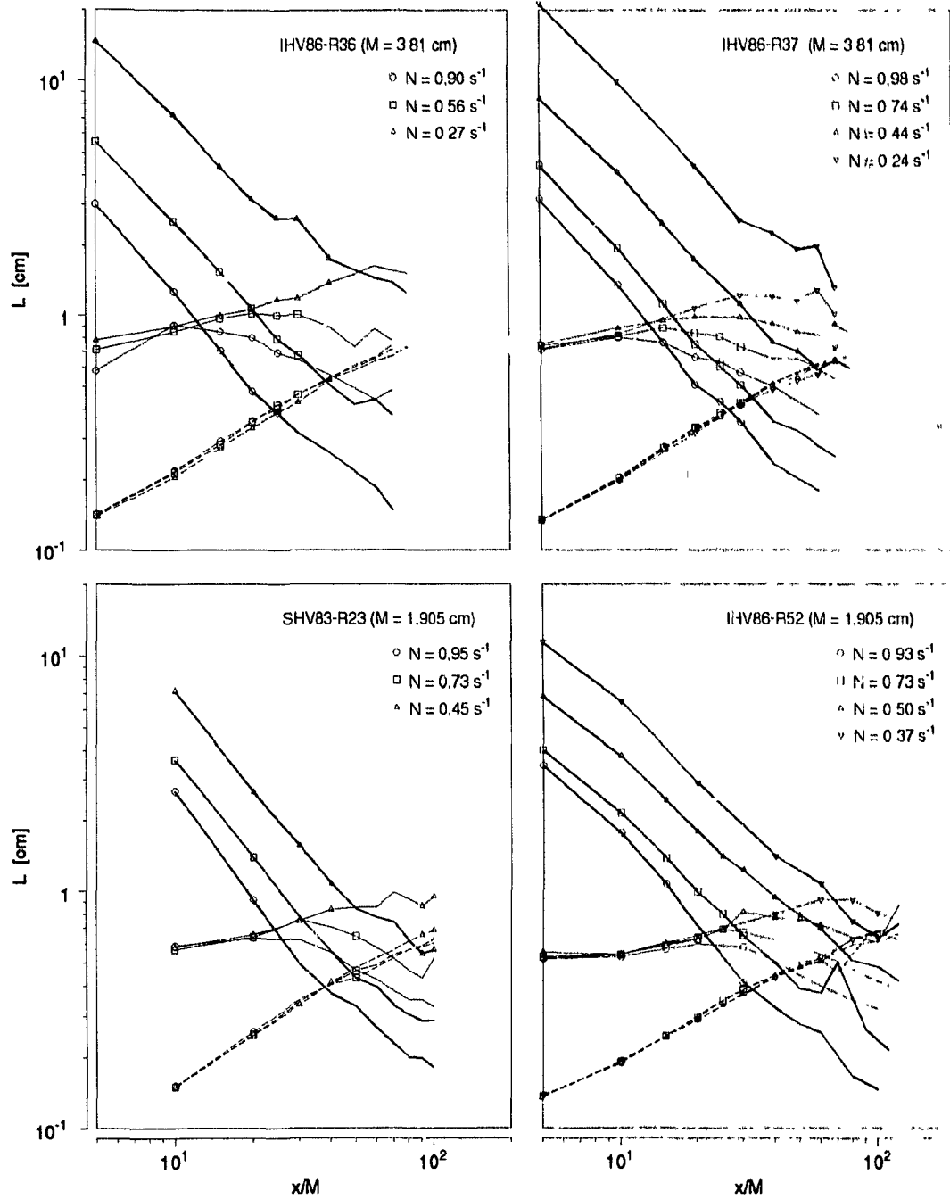
Figure 4.2: Evolution maps of turbulent length-scales for SHV and IHV experiments. Position is downstream of grid, non-dimensionalized by the grid mesh size M equal to 1.905 cm for R23 and R52 and 3.81 cm for R36 and R37. Group of lines are, from top to bottom, L_O (thick), L_t (thin) and 7.63 L_K for R36 and R37 and 9.86 L_K for R23 and R52 (dashed). Symbols were plotted only for data meeting the criterion q < 2.2(\epsilon L_t)^{1/3} explained in the text. Experiments evolve from left to right.
