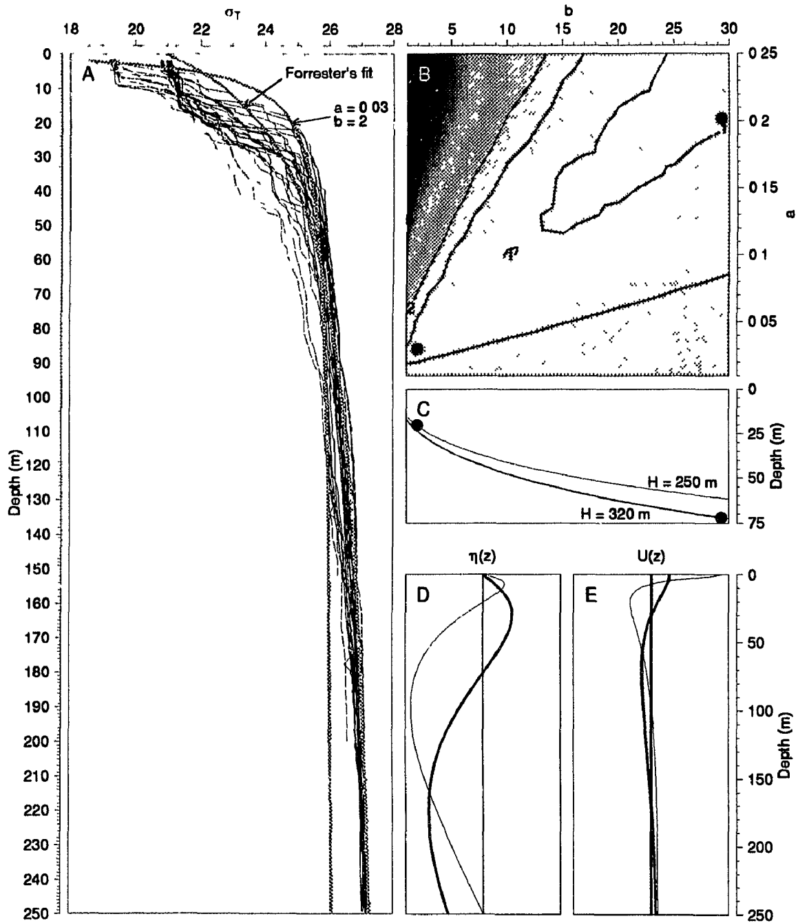
Figure 7.3: Mean density profile and its effect on node depth. A - Observed density profiles over nearly a tidal cycle at station 21 (solid) and 24 (dash) compared to Forrester's fit and an alternate fit; B - rms difference between observations and best fitting density profiles of a - b pairs. Dots shows a - b values for profiles in A; C - Depth of node of the second vertical mode for a channel of depth 320 m (thick) and 250 m (thin) as function of b ; D - Eigenfunction for isopycnal displacements, \eta , of the second vertical mode for Forrester's fit (thick) and b = 2 m (thin); E - Eigenfunction for velocity, d\eta/dz , of the second vertical mode for Forrester's fit (thick) and b = 2 m (thin).
