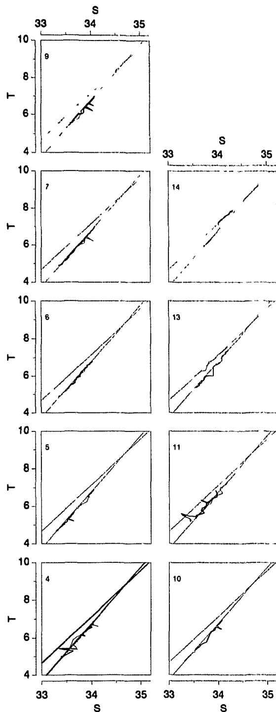
Figure 6.11: T - S diagram for all EPSONDE sequences preceded and followed by a CTD cast. The two lines are water masses traced on Figure 6.10. Sequence number indicated in upper left corner of each panel. Note that the finestructure density measurements in these CTD casts is unreliable; none of the apparent density inversions should be believed. In certain sequences, two end water masses are found at the start and end, such that intrusions could be present during the sequence. These intrusions, not observed in any way in this figure, could be seen as overturns by EPSONDE using only temperature profiles.
