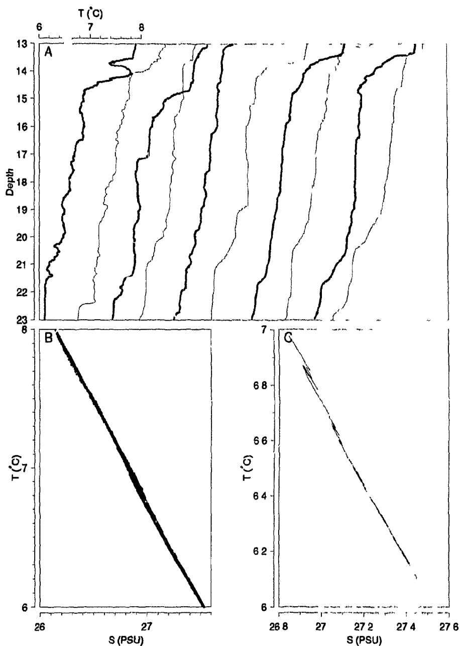
Figure 7.9: A - Temperature profiles for the 10 profiles of the mixing layer at station 11 discussed in the text and shown in the box in Figure 7.7. Only down traces of the CTD profiles are used. The profiles are shown alternatively with thin and thick line to better identify them; B - T - S diagram for the same 10 profiles; C - T - S diagram for part of the first profile. Note the tight relation even within overturning events.
