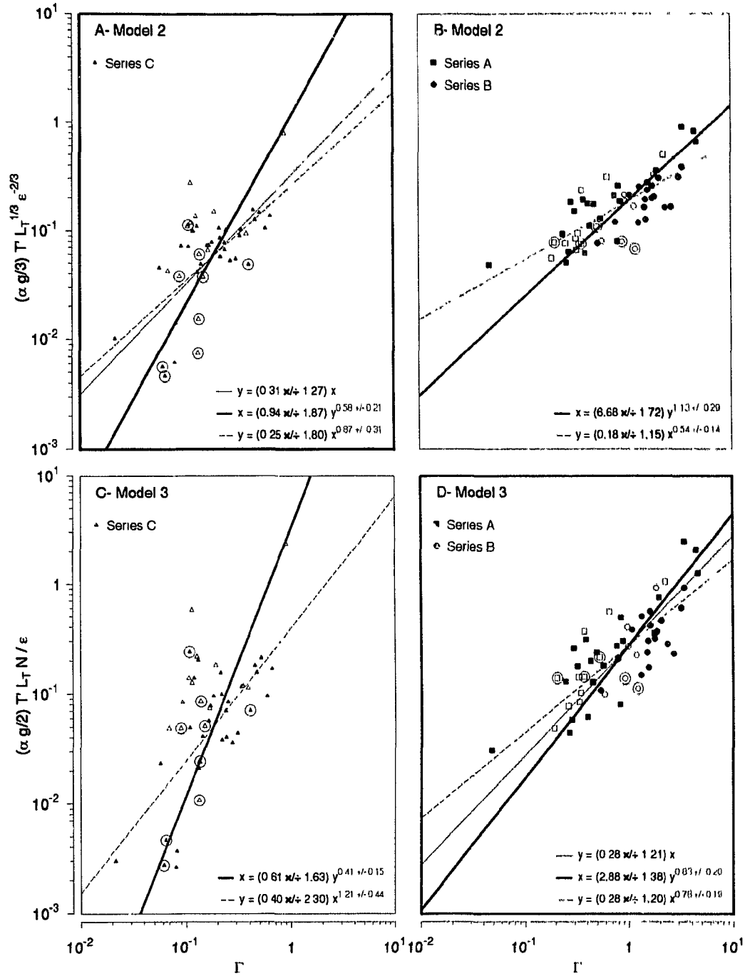
Figure 5.4: Mixing Efficiency compared to Models. A- Second model mixing efficiency prediction versus measure mixing efficiency for series C. GM regression has \Gamma_{model} \propto \Gamma^{1.2} ; B- Second model for series A and B. GM regression has \Gamma_{model} \propto \Gamma^{0.7} ; C- Third model for series C. GM regression has \Gamma_{model} \propto \Gamma^{1.7} ; D- Third model for series A and B. GM regression has \Gamma_{model} \propto \Gamma^{0.97} ; All regression are on data with \epsilon/\nu N^2 > 200 . Thick lines are x regressed on y ; thin lines are y regressed on x , solid lines have forced slope and dashed lines have best fitting slopes. Highlighted panels A and D indicate best fitting model.
