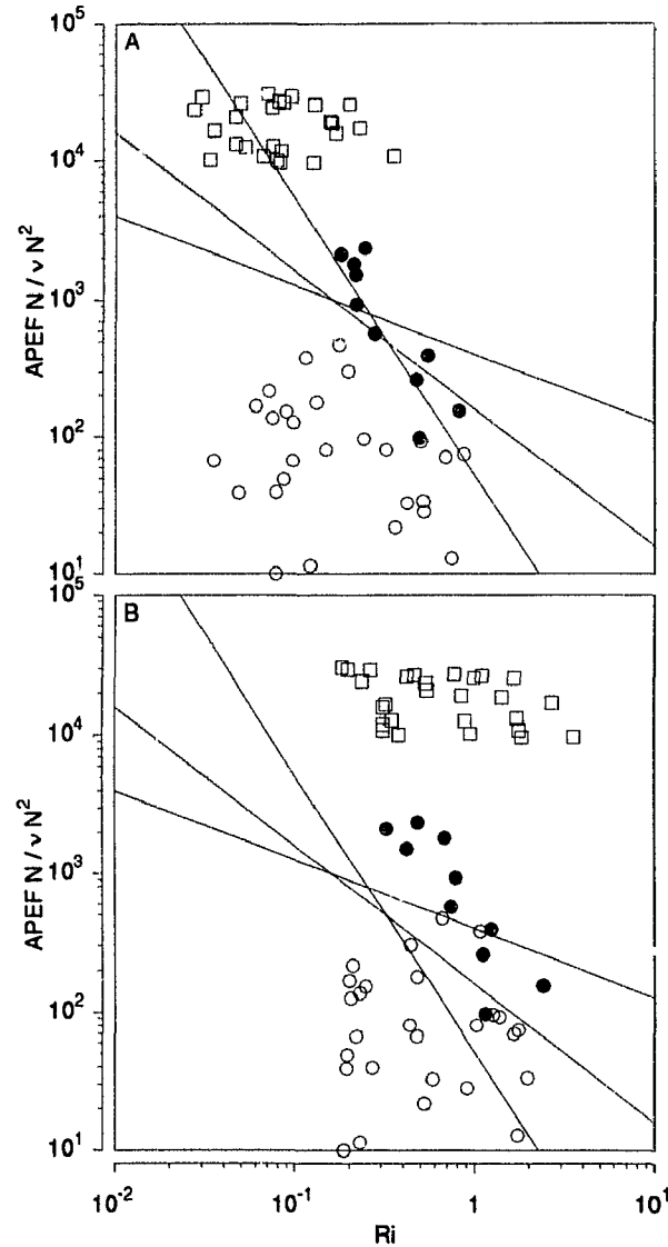
Figure 7.16: Comparison of Gregg's model with observed finestructure. A- \xi N versus minimum Ri_g in each 1-m thick time-average layer; B- \xi N versus log-averaged Ri_g in each 1-m thick layer; Data are from (●) new mixing layer, (○) well-mixed layer and (□) soliton. The lines are, from the steepest, combination of Gregg's model with the first model ( \epsilon = \xi N ), with the third model ( J_b = \xi N ) and with the second model ( J_b = (2/3)\xi N Fr_t ).
