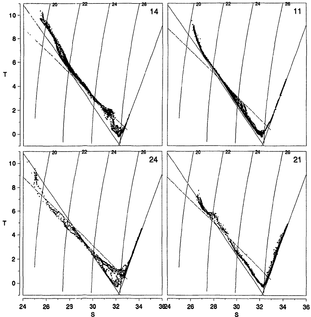
Figure 7.1: Temperature-Salinity Properties at the head of the Laurentian channel. Stations indicated in upper-right corner of each panel. Station locations are shown in Figure 7.2. Station 21 was sampled to 200 m every hour starting June 27 1988 15:01 EDT to June 28 04:58 EDT. Station 24 was also sampled to 200 m every hour, on June 29 from 14:01 to 22:59 EDT; Winds increased from very low to 25 knots at the end of the day. Station 14 was sampled to 50 m on July 4 from 04:50 to 14:04 EDT in 15 knot winds. Station 11 to 50 m was sampled from July 4 14:57 to July 5 02:45 in light winds. The last 3 profiles were taken to 235 m. See text for explanation of water mass lines.
