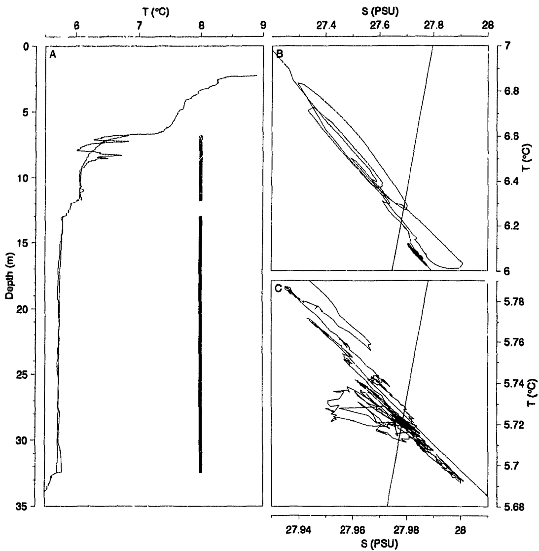
Figure 7.15: A - Measured and re-ordered temperature profile at 36.18 hours in Figure 7.10. The two vertical lines show the intervals of two overturns. B - T - S relation for top overturn in A. Oblique line is the \sigma_t = 21.75 isopycnal. C - T - S relation for bottom overturn in A. Oblique line is the \sigma_t = 22.04 isopycnal.
