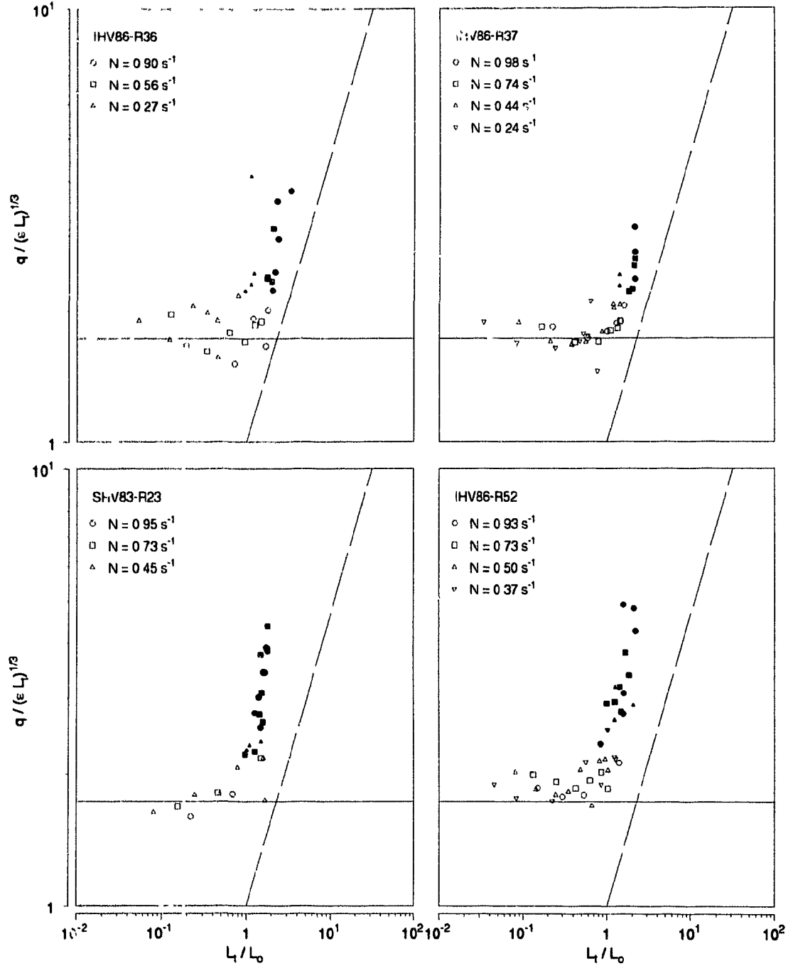
Figure 4.4: Internal waves detection criterion showing q/(\epsilon L_t)^{1/3} vs L_t/L_0 for all data from SHV and IHV experiments. The horizontal line is q/(\epsilon L_t)^{1/3} = 3^{1/2} which is approximately expected for isotropic turbulence. The dashed line is q/(\epsilon L_t)^{1/3} vs (L_t/L_0)^{2/3} , a relation expected for internal wave motions. Data with q/(\epsilon L_t)^{1/3} \geq 2.2 (filled symbols) are identified as internal waves because they resemble the q/(\epsilon L_t)^{1/3} \propto (L_t/L_0)^{2/3} criterion expected for internal waves rather than q/(\epsilon L_t)^{1/3} \approx 3^{1/2} expected for turbulence. Experiments evolve from left to right.
