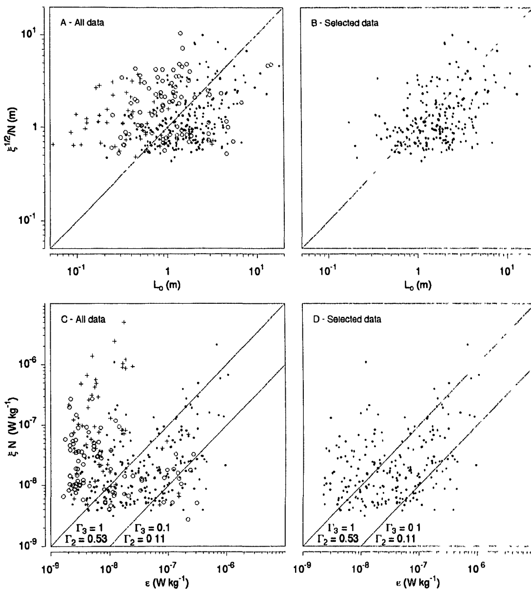
Figure 6.8: Buoyancy flux estimate \xi N versus dissipation \epsilon , and \xi^{1/2}N^{-1} vs L_0 for depth spans of well-resolved overturns, for all data set. In A and C , all data are plotted but are coded as: (+) shallower than 65 m; (o) between 8.6 and 9°C. Dots are all other data. In B and D , only dots from A and C are plotted (deeper than 65 m, yet not between 8.6 and 9°C). These well resolved data are have \overline{T'^2}^{1/2} > 0.003^\circ C and more than 3 points per overturn. Note that \xi^{1/2}N^{-1} approximates 0.707 L_T . The oblique line in A and B is a one-to-one line. The oblique lines in C and D are mixing efficiencies with the indicated values for the second and third models.
