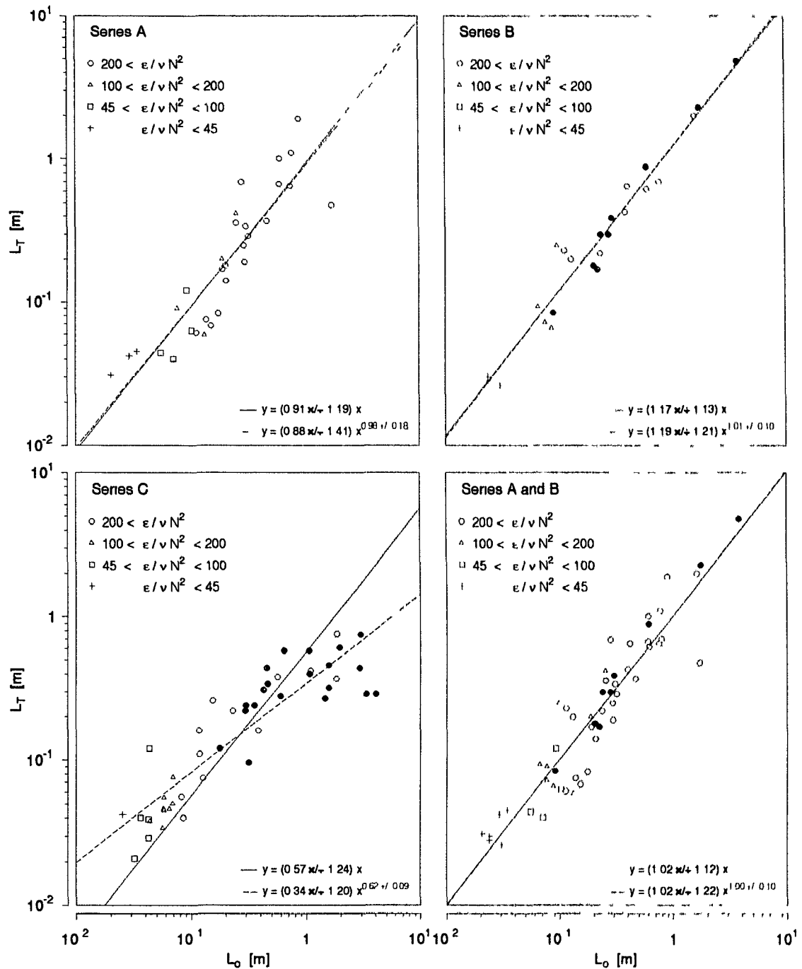
Figure C.1: Comparison of Thorpe scales L_T versus Ozmidov scales L_O for two oceanic cases (Series A and B) and a fresh water reservoir (Series C). Data are classified by turbulent intensity \epsilon / \nu N^2 . Open symbols are well resolved; filled symbols are marginally resolved. Data are from tables in Dillon (1982). This figure corresponds to Figures 8, 9 and 10 in Dillon (1982).
