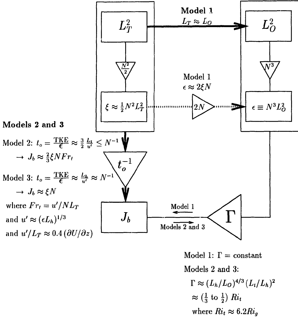
Figure 3.1: Diagram of the three models derived in this chapter. Model one: Traditional view linking L_T to L_O , and therefore \xi to \epsilon via a decay time N^{-1} . A constant mixing efficiency is assumed; Model two: New model for growing isotropic turbulence, linking \xi to J_b via a decay time \propto L_T/u' \propto (\partial \bar{U}/\partial z)^{-1} ; Model three: New model for anisotropic inertial-buoyancy balanced turbulence, linking \xi to J_b via a decay time N^{-1} ; Mixing efficiency for models two and three depend on Ri_t , which can be inferred from Ri_g or \epsilon and \xi N . Boxes indicate measurable quantities, and triangles are multipliers that relate those quantities to each other.
