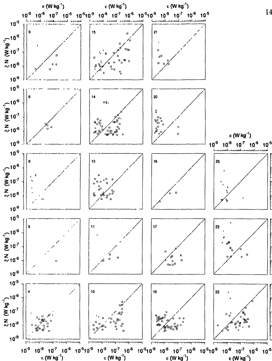
Figure 6.9: Overturn-averages of \epsilon N vs \epsilon for individual EPSONDE sequences. (+) shallower than 65 m; (o) between 8.6 and 9°C; (□) all other data. Sequence number indicated in upper left corner of each panel. Oblique line is mixing efficiency \Gamma_2 = 0.53 or \Gamma_3 = 1 .
