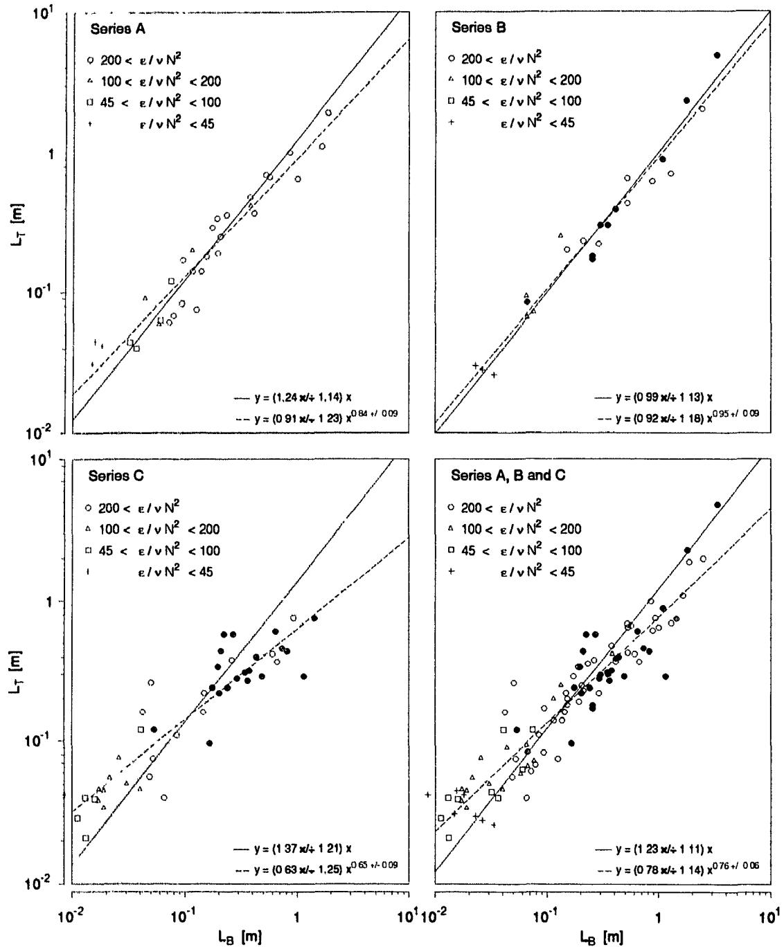
Figure C.2: Comparison of L_T vs L_B for two oceanic cases (Series A and B) and a fresh water reservoir (Series C). Data are classified by turbulent intensity \epsilon/\nu N^2 . Open symbols are well resolved; filled symbols are marginally resolved. Data are from tables in Dillon (1982). This figure corresponds to Figure 11 in Dillon (1982).
