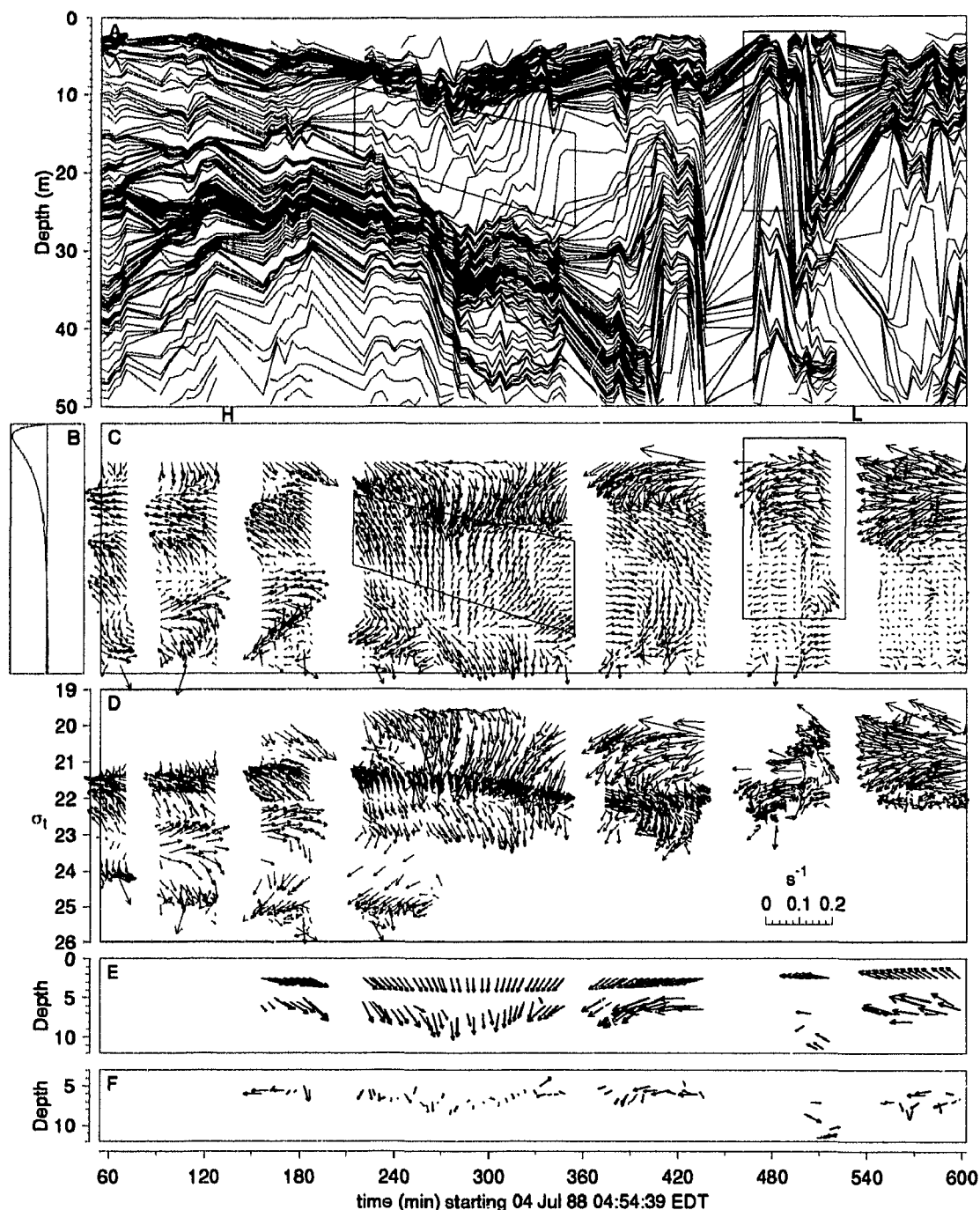
Figure 7.6: Shear and isopycnal displacements at Station 14. A - Isopycnal displacement obtained from CTD casts sampled approximately every 4 minutes, collected at the same time as the shear vectors of panel C; B - Theoretical Poincaré shear depth-modulation for n = 2 , b = 2 m and H = 250 m; C - Shear vectors from 0 to 32 m. Towards the right is down-channel and downwards is toward the South side of the channel. Scale indicated in panel D; D - Shear plotted against density; E - Bottom arrows: average shear for \sigma_t < 21 . Top arrows: Tidal-frequency rotating vector least-squares fit to bottom arrows; F - Difference between average shear and fit in panel E; Boxed areas in A and C indicate mixing layers described in later sections. Letters H and L between panels A and C indicate high and low tide.
