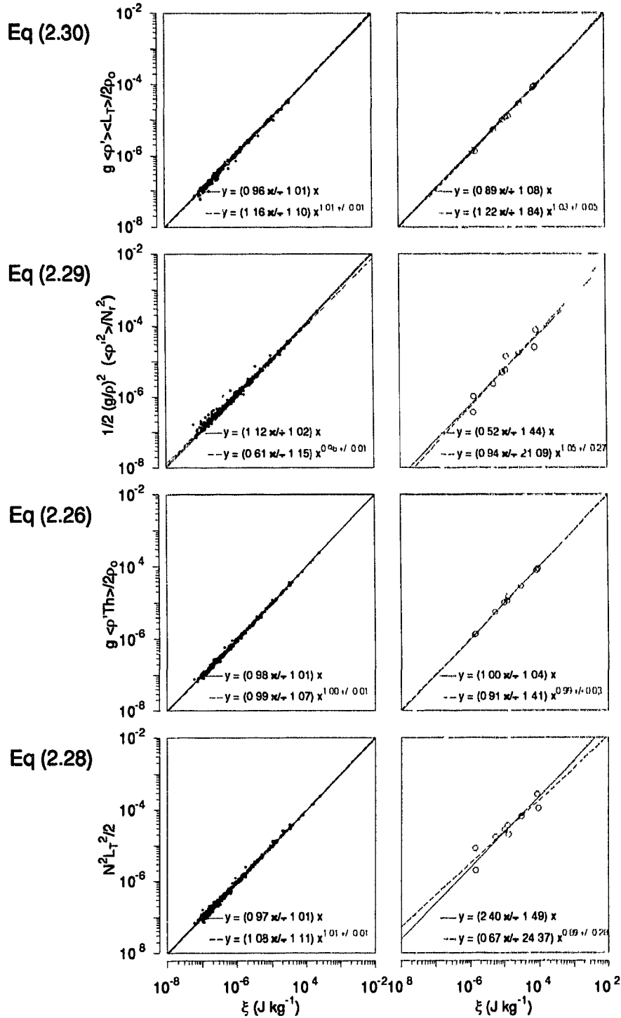
Figure 2.1: Four approximations of the APEF, \xi , are evaluated using data from 9 CTD casts in the St. Lawrence estuary. The panels on the left are calculated using statistics averaged over individual overturns; those on the right used one average per profile over the entire layer.
