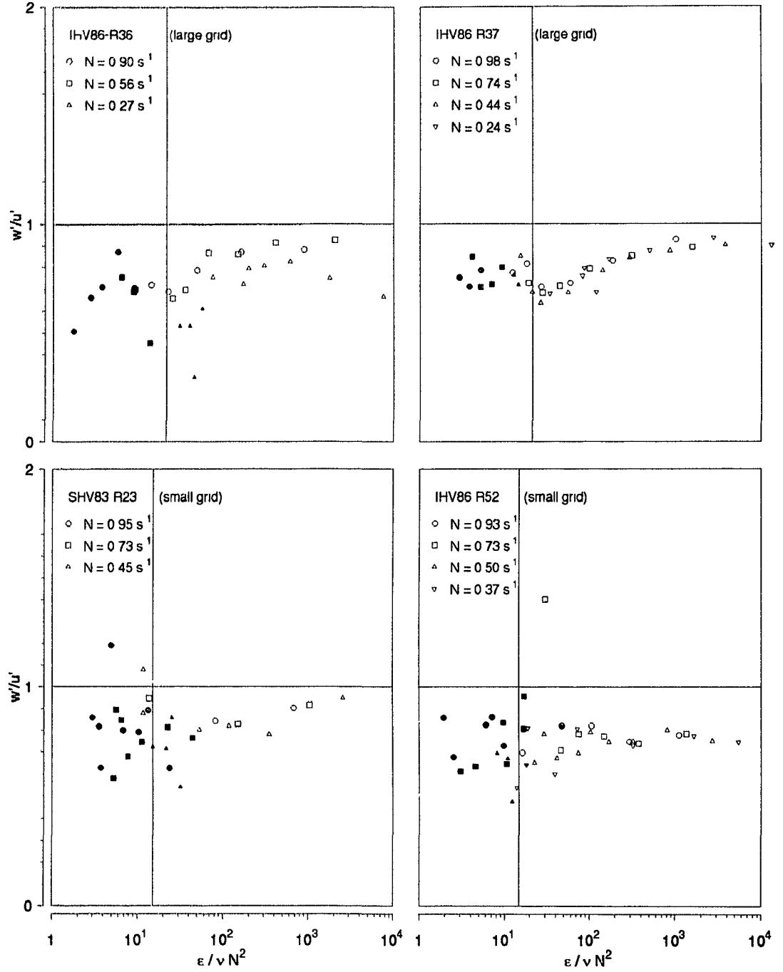
Figure A.1: Isotropy of rms turbulent velocities w'/u' versus turbulence intensity \epsilon/\nu N^2 . Values in the legend are for N in \text{s}^{-1} . Open symbols are for q/(\epsilon L_t)^{1/3} < 2.2 (turbulence) and solid symbols for q/(\epsilon L_t)^{1/3} \geq 2.2 (internal waves). The vertical lines are for \epsilon/\nu N^2 = 15 (small grid mesh size) and \epsilon/\nu N^2 = 21 (large grid mesh size). They are the values quoted by Itsweire et al. (1986) at which buoyancy flux ceased.
