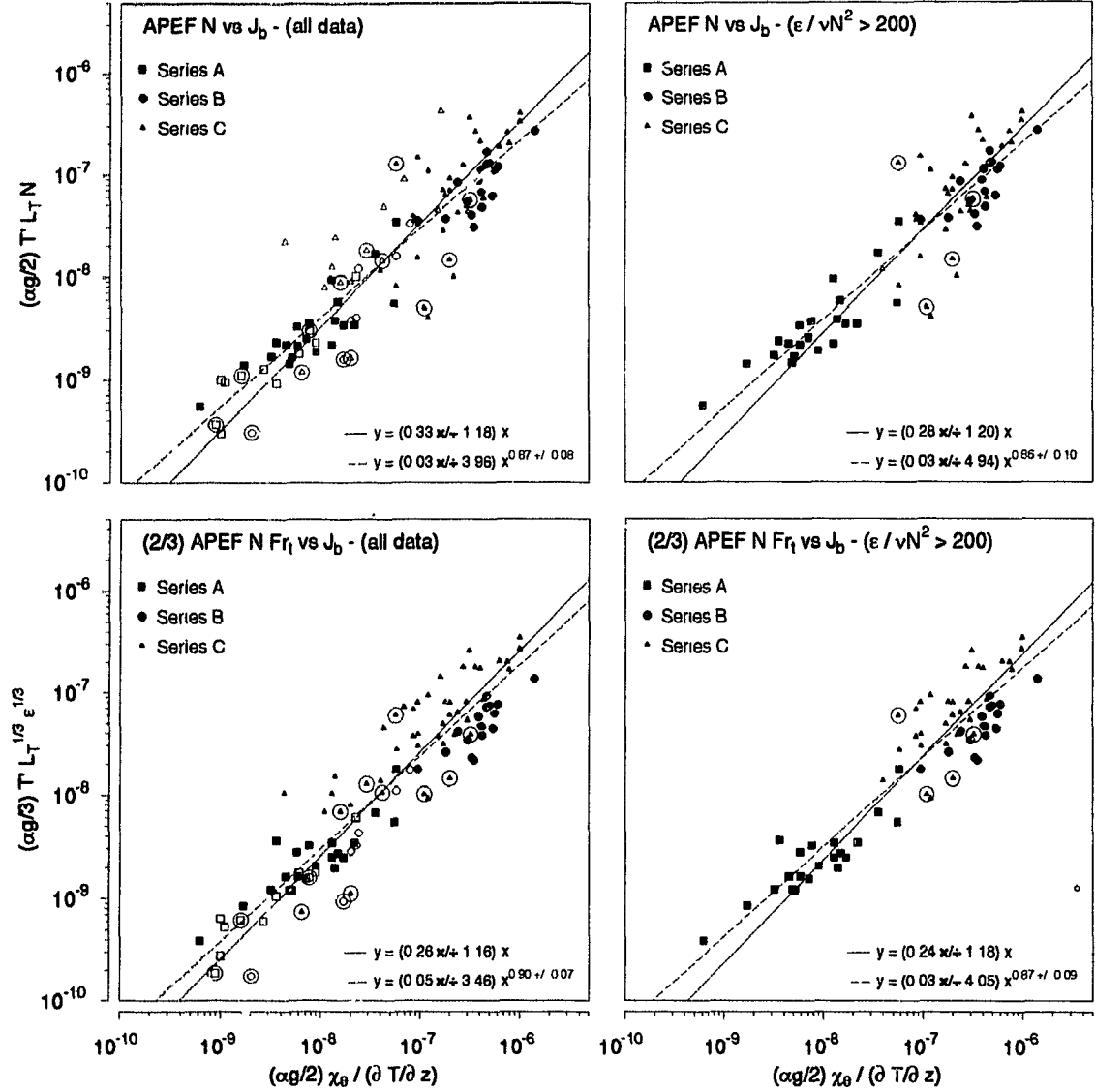
Figure 5.3: Comparison of two derivations of the buoyancy flux models from Chapter 3. The top two panels compare (\xi N) to J_b approximating \xi as (\alpha g/2) \overline{T}^{1/2} L_T (and J_b is approximated by the dissipation of potential energy in all panels). The bottom panels compare ((2/3)\xi N Fr_t) to J_b , where (2/3)\xi N Fr_t is best approximated by (\alpha g/3) \overline{T}^{1/2} L_T^{1/3} \epsilon^{1/3} for Dillon's tabled data. Data are coded by the data set, by turbulent intensity (open symbols have \epsilon/\nu N^2 < 200 ; solid symbols have \epsilon/\nu N^2 > 200 ) and circled data have (\overline{T}^{1/2}/L_T)/(\partial \overline{T}/\partial z) < 0.2 . The left-hand side panels include all data and the right-hand side ones include only data with \epsilon/\nu N^2 > 200 .
