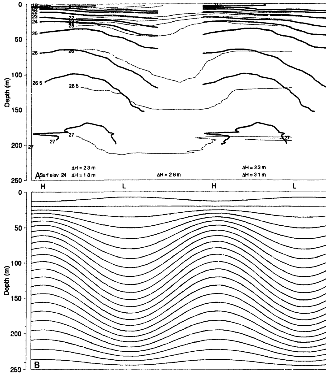
Figure 7.4: A- Isopycnal displacements for station 21 (thin line) and 24 (thick line) vs tidal phase. Station 24 is shown twice to better compare it with station 21. The tidal elevations indicated are surface elevation differences between high and low tides. High tide is indicated by H, low tide by L; B- Theoretical isopycnal oscillations for the second vertical mode with density profile described by (7.2) with b = 2 m. The phase with respect to the barotropic tide is not determined, and can be offset in panel A. The inversions on both series at high tide is due to overturning in both cases.
