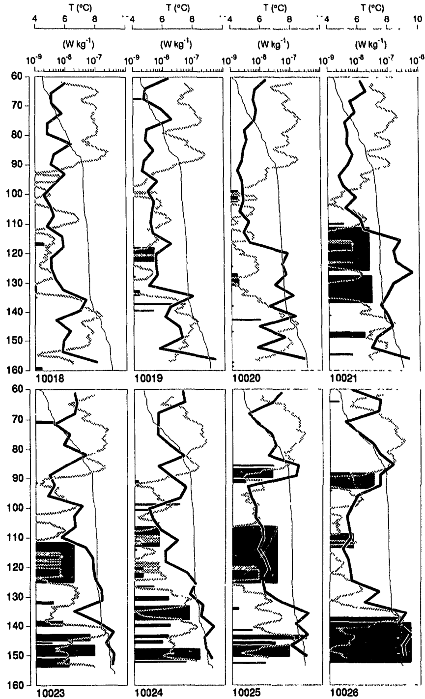
Figure 6.5: Noise level for \xi N in 10018–10026 sequence. The thick gray line is the noise level for \xi N . The thick black line is \epsilon . Overturns are not expected to be observed if \epsilon is less than the noise level. The black rectangles span the depth of overturns and their width represents \xi N for the overturn. These quantities are on a logarithmic scale of 10^{-9} to 10^{-6} W kg -1 . The temperature profile is also plotted (thin line).
