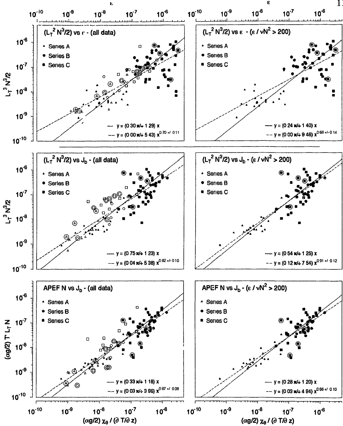
Figure 5.2: Comparison of models inferred from Dillon's results. The top two panels compare (L_T^2 N^3/2) to \epsilon . The middle two compare (L_T^2 N^3/2) to the estimated buoyancy flux. The bottom two compare (\xi N) to estimated J_b approximating \xi as (\alpha g/2) \overline{T'^2}^{1/2} L_T . Data are coded by the data set, by turbulent intensity (open symbols have \epsilon/\nu N^2 < 200 ; solid symbols have \epsilon/\nu N^2 > 200 ) and circled data have (\overline{T'^2}^{1/2}/L_T)/(\partial \overline{T}/\partial z) < 0.2 . The left-hand side panels include all data and the right-hand side ones include only data with \epsilon/\nu N^2 > 200 .
