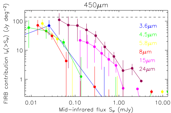
Figure 17. Cumulative contributions to the 450 \mu\text{m} extragalactic background light, as a function of near/mid-infrared flux, for various Spitzer/ISO surveys. Symbols as figure 16. Note that the Spitzer contributions are capable of accounting for the entire 450 \mu\text{m} background, within the errors.
