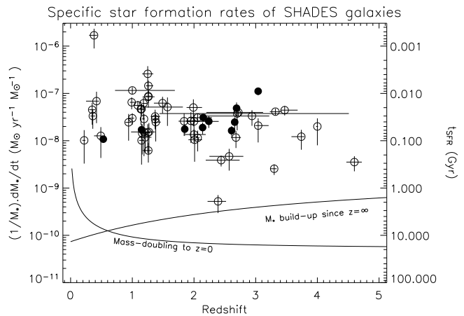
Figure 13. Star formation rate per unit galaxy mass, (1/M)dM/dt , for the SHADES point sources in the Lockman Hole. As with figure 12, the corresponding star formation timescales are given in the right-hand ordinate. Objects with spectroscopic redshifts are shown in filled symbols, and objects with optical-Spitzer-based photometric redshifts from Dye et al. (2008) are shown as open symbols. Note that the star formation timescales for SHADES sources are much shorter than in the population as a whole.
