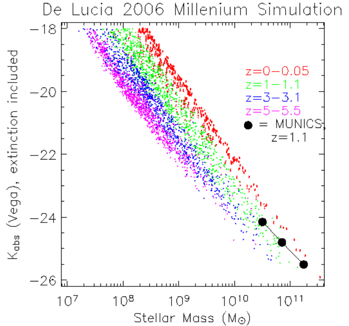
Figure 2. Correlation between model stellar mass and absolute K magnitude predicted using the Millenium simulation by de Lucia (2006), for several redshift shells. Also plotted are the data from the MUNICS survey (Drory et al. 2004). Note the small dispersion and the clear redshift dependence.
