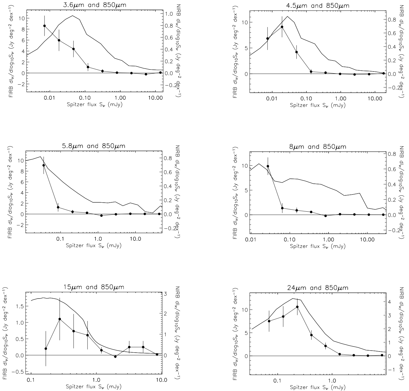
Figure 14. Contributions of the Spitzer/ISO galaxies to the 850\ \mu\text{m} extragalactic background light (data points, left-hand ordinates) as a function of Spitzer/ISO flux. Also plotted are the contributions of the same galaxies to the cosmic near-infrared and mid-infrared backgrounds (curves, right-hand ordinates), estimated from the source counts as discussed in the text. Note in particular the correspondence between the 24\ \mu\text{m} and 850\ \mu\text{m} extragalactic backgrounds.
