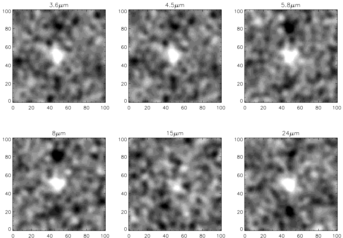
Figure 9. Signal-to-noise images of stacked 450\ \mu\text{m} postage stamps centred on Spitzer/ISO galaxies, as discussed in the text. The greyscale is from -3\sigma to +4\sigma . The scales marked are arcseconds. Note the clear detections at the centres of all the images. Negative sidelobes are also visible.
