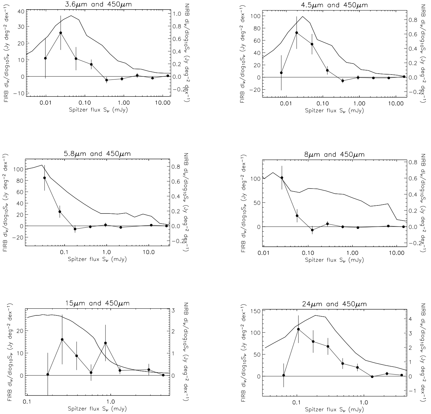
Figure 15. Contributions of the Spitzer/ISO galaxies to the 450\ \mu\text{m} extragalactic background light (data points, left-hand ordinates) as a function of Spitzer/ISO flux. Also plotted are the contributions of the same galaxies to the cosmic near-infrared and mid-infrared backgrounds (curves, right-hand ordinates), estimated from the source counts as discussed in the text. Note in particular the correspondence between the 3.6 - 4.5\ \mu\text{m} and 450\ \mu\text{m} extragalactic backgrounds.
