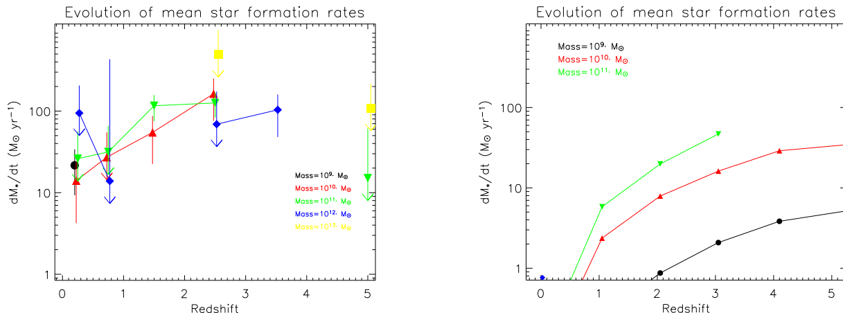
Figure 11. Left: mean star formation rates, dM_*/dt , of our galaxies. Symbols as in figure 10. Right: corresponding predictions from the de Lucia et al. (2006) simulation. Note that the observed star formation rates clearly exceed the predictions.
