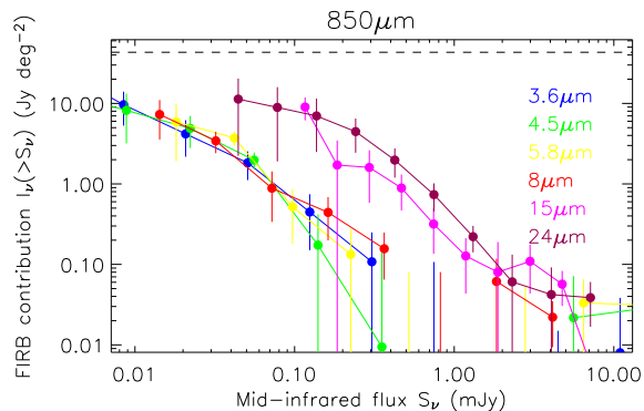
Figure 16. Cumulative contributions to the 850 \mu\text{m} extragalactic background light, as a function of near/mid-infrared flux, for various Spitzer/ISO surveys. The horizontal dashed line is the total background derived by Lagache et al. (1999), the uncertainties on which are less than a factor of 2. Note that the Spitzer contributions converge to roughly a quarter of the total 850 \mu\text{m} background.
