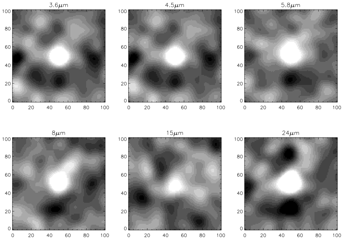
Figure 8. Signal-to-noise images of stacked 850\ \mu\text{m} postage stamps centred on Spitzer/ISO galaxies, as discussed in the text. The greyscale is from -3\sigma to +4\sigma . The scales marked are arcseconds. Note the clear detections at the centres of all the images. Negative sidelobes are also visible.
