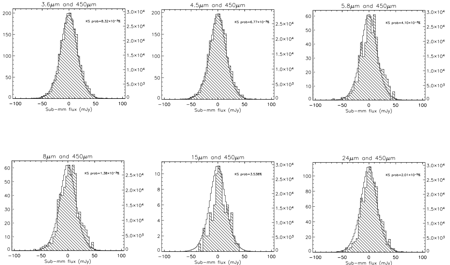
Figure 7. Histograms of 450\ \mu\text{m} flux in the SHADES Lockman map as a whole (unhatched bars) compared to the 450\ \mu\text{m} fluxes at the positions of the Spitzer/ISO galaxies selected at the indicated wavelengths (hatched bars). The left-hand vertical scales show the numbers for the hatched histograms, and the right-hand scales refer to the unhatched histograms. Note that in all plots, the hatched bars lie typically to the right of the unhatched bars. The results of a comparison using the Kolmogorov-Smirnoff test are also shown in the diagrams.
