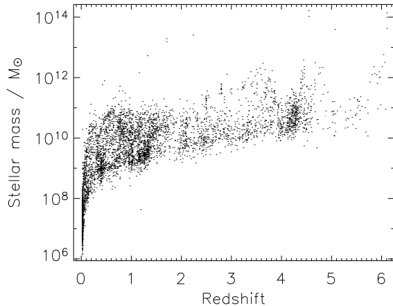
Figure 3. Model stellar mass estimates of Spitzer galaxies discussed in the text, versus photometric redshifts from Dye et al. (2008, SHADES paper VII). Note that the model stellar masses above z = 0.5 depend only weakly on photometric redshift.
