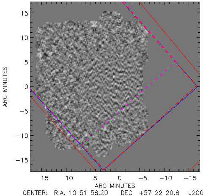
Figure 1. The SHADES 850\ \mu\text{m} map with point sources subtracted, used for stacking analyses in this paper (greyscale). Also plotted is the coverage of the Spitzer 24\ \mu\text{m} data (solid red line), the 3.6\ \mu\text{m} data (solid blue line), 4.5\ \mu\text{m} (solid green line), 5.8\ \mu\text{m} (dashed red line), and 8\ \mu\text{m} (dashed magenta line). Note the availability of Spitzer data over most of the SHADES area.
