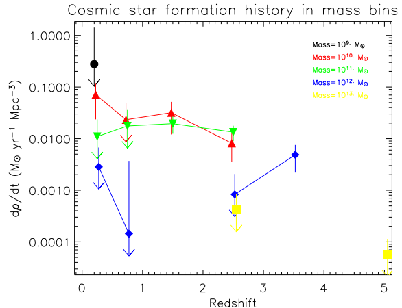
Figure 10. Evolution in comoving volume-averaged star formation rates as a function of total mass for 3.6\ \mu\text{m} -selected galaxies, in \pm 0.5 dex mass bins centred on the masses shown. The brighter submm point source population discovered by Smail et al. 1997, Hughes et al. 1998 and Barger et al. 1998 are not included, because we removed submm point sources prior to our stacking analysis. Symbols: the circle is 10^9 M_\odot , upward triangles 10^{10} M_\odot , downward triangles 10^{11} M_\odot , diamonds 10^{12} M_\odot , and the square is the 10^{13} M_\odot constraint. Note that the lower-mass galaxies have star formation histories peaking at much lower redshifts than the putative z \simeq 2.2 peak in the bright submm point source population.
