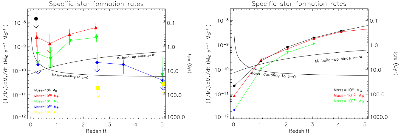
Figure 12. Left: star formation rate per unit galaxy mass, (1/M)dM/dt . This has dimensions of [T]^{-1} and the corresponding star formation timescales are given in the right-hand ordinate. Symbols as in figure 10. Also plotted is the specific star formation rate required to double the stellar mass by z = 0 assuming a constant specific star formation rate, and the rate required to assemble the galaxy since the Big Bang assuming a constant star formation rate. Points lying above either line may be regarded as starbursting. Note that most of our detections can be regarded as starbursting. Right: corresponding predictions from the de Lucia et al. (2006) simulation. Note the obvious discrepancies with the observations.
