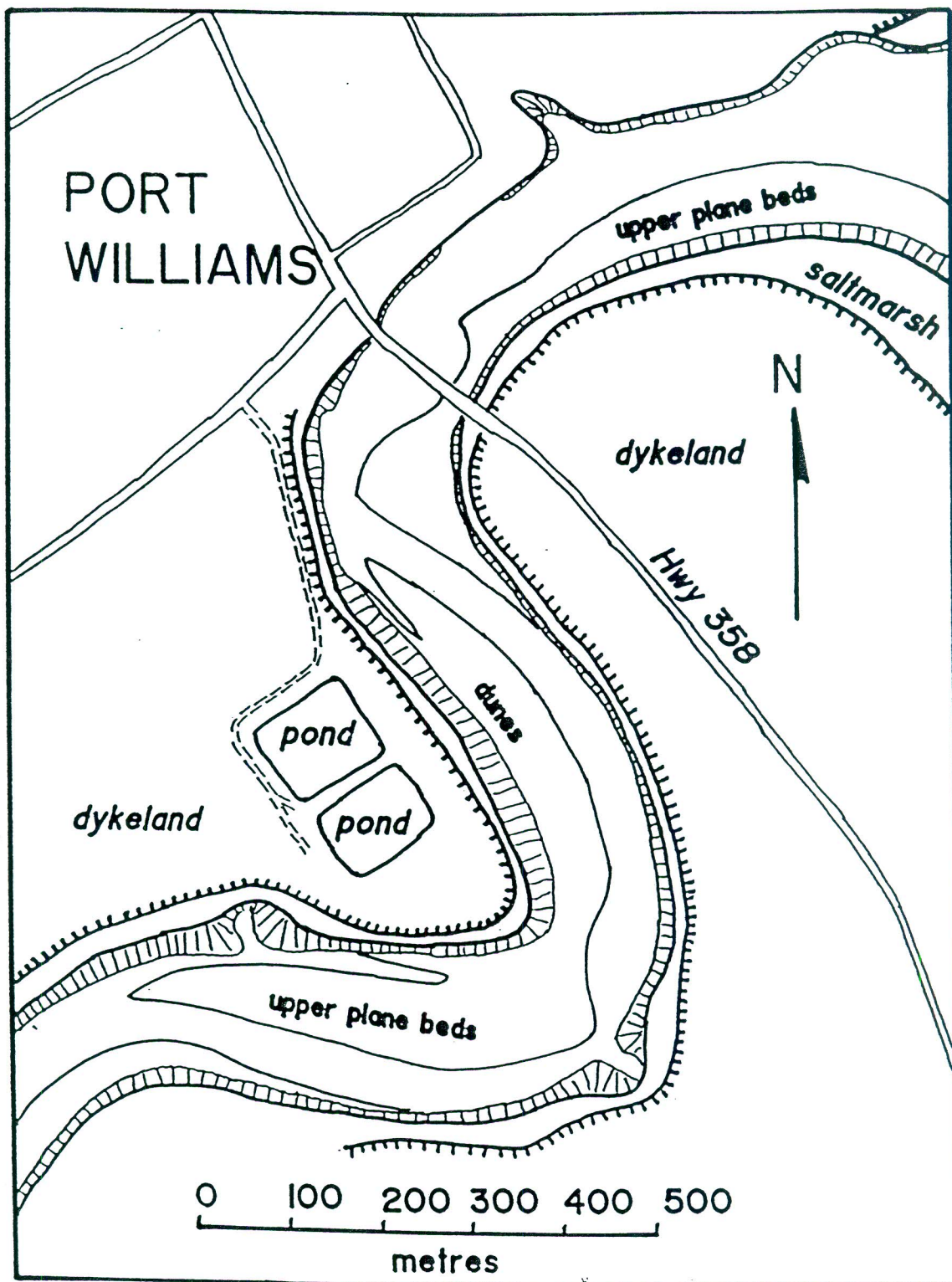
Figure 6. Sketch map of the Cornwallis River at the Port Williams bridge.
