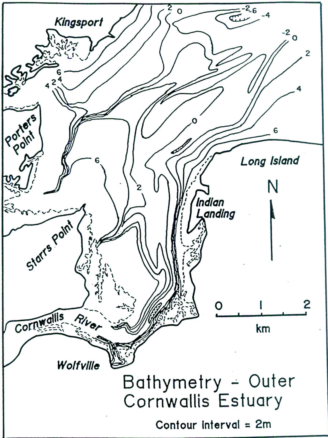
Figure 3. Bathymetry of the outer Cornwallis River. Datum is approximately mean low water. Note the development of flood "barbs" along the west side of the Cornwallis channel.
