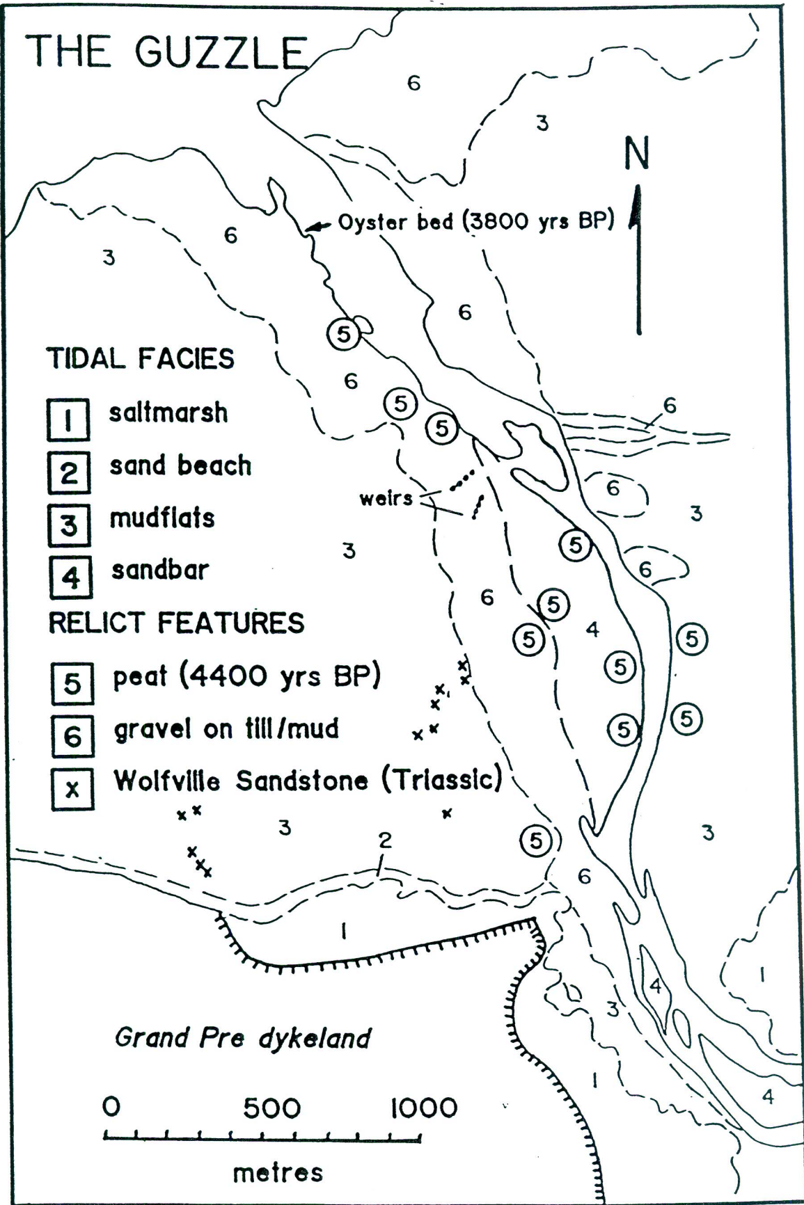
Figure 5. Sketch map of The Guzzle area at Evangeline Beach showing the distribution of major facies and features.
