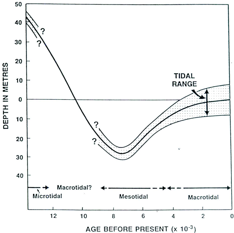
Figure 2(b). History of sea level and tidal range in the inner Bay of Fundy, based on data from Chignecto Bay (after Amos and Zaitlin, 1985). A similar pattern of sea-level and tidal range oscillations have occurred in the Minas Basin but with smaller amplitudes.
