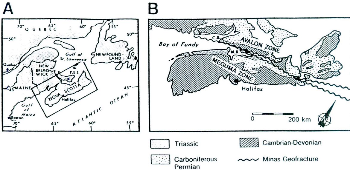
Figure 2(a). A: Location map of eastern Canada B: Geological and location map of the Bay of Fundy region. M.B.- Minas Basin; C.B. Chignecto Bay.
