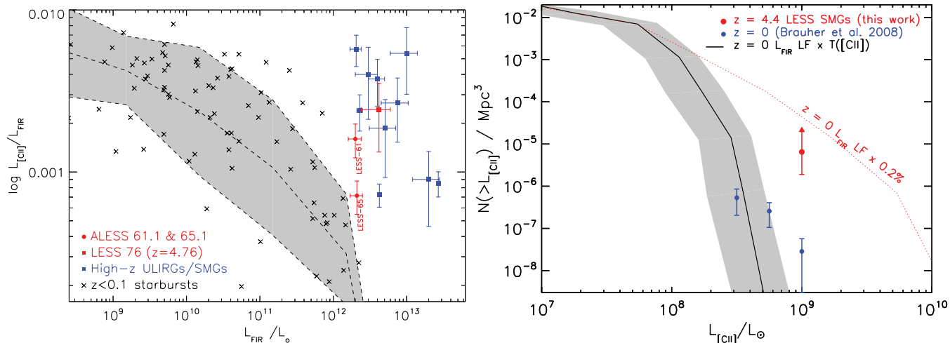
Figure 5. Left: L_{[\text{C II}]} / L_{\text{FIR}} ratio as a function of the far-infrared luminosity for our two z=4.4 ALMA SMGs compared to local star-forming galaxies and ULIRGs. In the plot we also include the z=4.76 LESS SMG from De Breuck et al. (2011; see also Coppin et al. 2009). We also include a number of high-redshift starbursts and AGN from previous studies (Carral et al. 1994; Luhman et al. 1998, 2003; Colbert et al. 1999; Unger et al. 2000; Malhotra et al. 2001; Spinoglio et al. 2005; Brauher et al. 2008; Stacey et al. 2010; Cox et al. 2011). For the local data, we calculate the median (dashed line) and scatter (grey). This figure shows that the ratio of L_{[\text{C II}]} / L_{\text{FIR}} for high-redshift ULIRGs is a factor of \sim 10 times higher given their far-infrared luminosities compared to those at z \sim 0 . Right: the [C II] luminosity function at z=4.4 from our survey compared to z=0 . For the z=4.4 luminosity function, we assume that all of the [C II]-emitting galaxies in the \Delta z=0.12 volume covered by our observations were detected and so we stress that these calculations yield only a lower limit on the volume density of high-redshift [C II] emitters. The z=0 observations are derived from volume density of IRAS sources at z < 0.05 from Brauher et al. (2008). The red dotted line shows the predicted [C II] local luminosity function for a constant L_{[\text{C II}]} / L_{\text{FIR}} = 0.002 , whilst the solid line shows the z=0 far-infrared luminosity function convolved with the L_{[\text{C II}]} / L_{\text{FIR}} function from Brauher et al. (2008) (with the grey region denoting the errors in the volume density of local ULIRGs and scatter in the transfer function). Finding two galaxies in this volume probed by our observations indicates a factor of \gtrsim 1000 increase in the number density of luminous [C II] emitters from z \sim 0 to 4.4, equivalent to an \sim 3 –4 times [C II] luminosity evolution between z=0 and 4.4.
