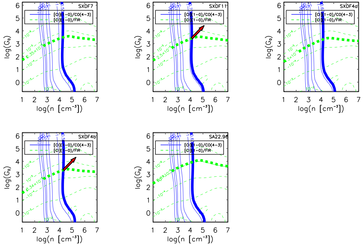
Figure A1. Contours of L_{[\text{CI}](1-0)}/L_{\text{CO}(4-3)} (solid blue) and L_{[\text{CI}](1-0)}/L_{\text{FIR}} (dashed green) at various levels of gas density ( n ) and radiation field ( G_0 ) from the Photo-Dissociation Region (PDR) models of Kaufman et al. (1999). The bold contours represent the observed ratios for each of the SMGs with new [CI] detections presented in this work. The intersection of the two contours in each case provides a value for n and G_0 for the SMG system. The red arrows mark the sources where there is only a limit to the [CI](1-0) luminosity and therefore we can only gain a lower limit to n and G_0 .
