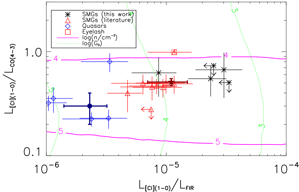
Figure 8. Luminosity ratios (in units of L_{\odot} ) of the SMGs in this work and in the literature compared to the quasar sample with [CI] detections detailed in Walter et al. (2011). The median values for the complete SMG and quasar samples are marked by the dark red filled star and dark blue filled circle respectively. The SMGs have higher L_{[CI](1-0)}/L_{FIR} and L_{[CI](1-0)}/L_{CO(4-3)} ratios than the literature sample of quasars. The contours plotted indicate the derived values of the gas density ( n ) and the radiation field ( G_0 ) for the corresponding ratios of L_{[CI](1-0)}/L_{CO(4-3)} and L_{[CI](1-0)}/L_{FIR} from PDR model outputs as detailed in Section 4.3. However, we note that if only a small fraction of the [CI] emission is due to the PDRs (Section 4.3.1) then all the ratio values should be lower than plotted (since the non-PDR contribution to the [CI] emission should be subtracted from the observed values) therefore suggesting higher densities and radiation field values for the PDR-related gas. Furthermore, assuming that the [CI] is non-PDR distributed and instead traces the bulk H_2 gas mass this plot shows compact starbursts in the low L_{[CI](1-0)}/L_{FIR} and L_{[CI](1-0)}/L_{CO(4-3)} region since the ^{12}CO(4-3) and far-infrared luminosities trace the same gas as the [CI], and systems with extended gas distributions in the high L_{[CI](1-0)}/L_{FIR} and L_{[CI](1-0)}/L_{CO(4-3)} region where the [CI] traces the star-formation idle H_2 gas but the ^{12}CO(4-3) and far-infrared trace the star-forming gas only.
