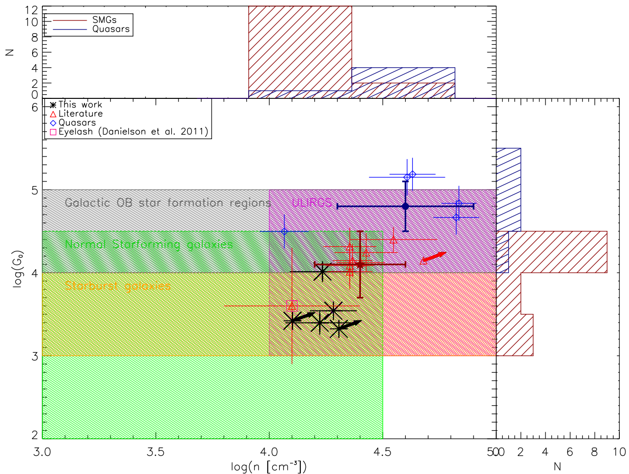
Figure 9. The far-UV radiation field, in terms of the local value ( G_0 ), against the gas density ( n ) derived from the comparison of various [CI], ^{12}\text{CO} and far-infrared luminosities to the outputs from the Kaufman et al. (1999) PDR models. We plot the derived values for the SMGs and the literature quasars. The median values for the complete SMG and quasar samples are marked by the dark red filled star and dark blue filled circle respectively. We also mark the ranges in n and G_0 derived for other populations - local ULIRGs, Galactic OB star-formation regions, normal star-forming galaxies and starburst galaxies (Stacey et al. 1991; Malhotra et al. 2001; Davies et al. 2003). We find that the SMGs are most comparable to the local ULIRGs although the tail of 5 SMGs with lower densities and radiation field values are more consistent with local starburst galaxies.
