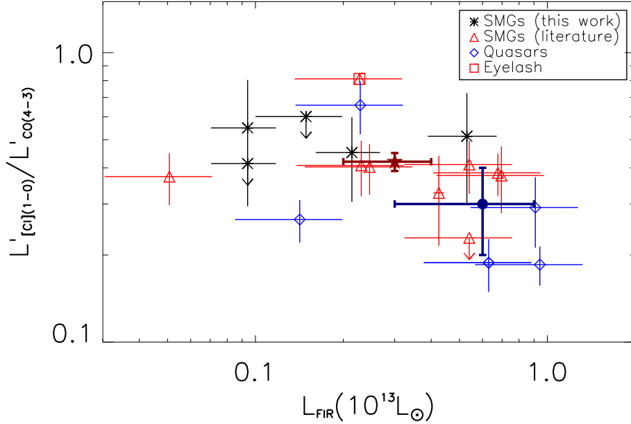
Figure 7. Line luminosity ratios and far-infrared luminosities of the SMGs in this work and in the literature compared to the sample of quasars with [CI] detections detailed in Walter et al. (2011). All luminosities are corrected for gravitational lensing using the magnification factors in Table 5. The ratio of L'_{[CI](1-0)}/L'_{CO(4-3)} decreases with increasing far-infrared luminosity. The median values for the complete SMG and quasar samples are marked by the dark red filled star and dark blue filled circle respectively. The SMGs extend to higher L'_{[CI](1-0)}/L'_{CO(4-3)} and lower L_{FIR} values than the quasar sample. The ratio of L'_{[CI](1-0)}/L'_{CO(4-3)} decreases with increasing L_{FIR} . Assuming that the [CI] provides a tracer of the bulk H_2 gas mass, in merger systems (with higher L_{FIR} values) a larger fraction of bulk H_2 gas will participate in the star-formation therefore the ratio of L'_{[CI](1-0)}/L'_{CO(4-3)} will be reduced compared to systems with extended distributions of star-formation idle H_2 gas which will have higher values of L'_{[CI](1-0)}/L'_{CO(4-3)} and lower L_{FIR} values.
