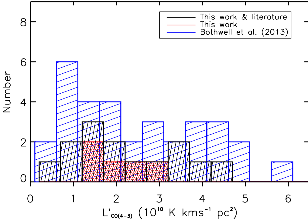
Figure 6. The distribution of L'_{\text{CO}(4-3)} of the SMGs with new [C1] detections in this work (red dense shading) and the combination of this sample and the literature sample of SMGs with [C1] detections (black medium shading) compared to the large sample of SMGs which have been studied in ^{12}\text{CO} by Bothwell et al. (2013) (blue sparse shading).
