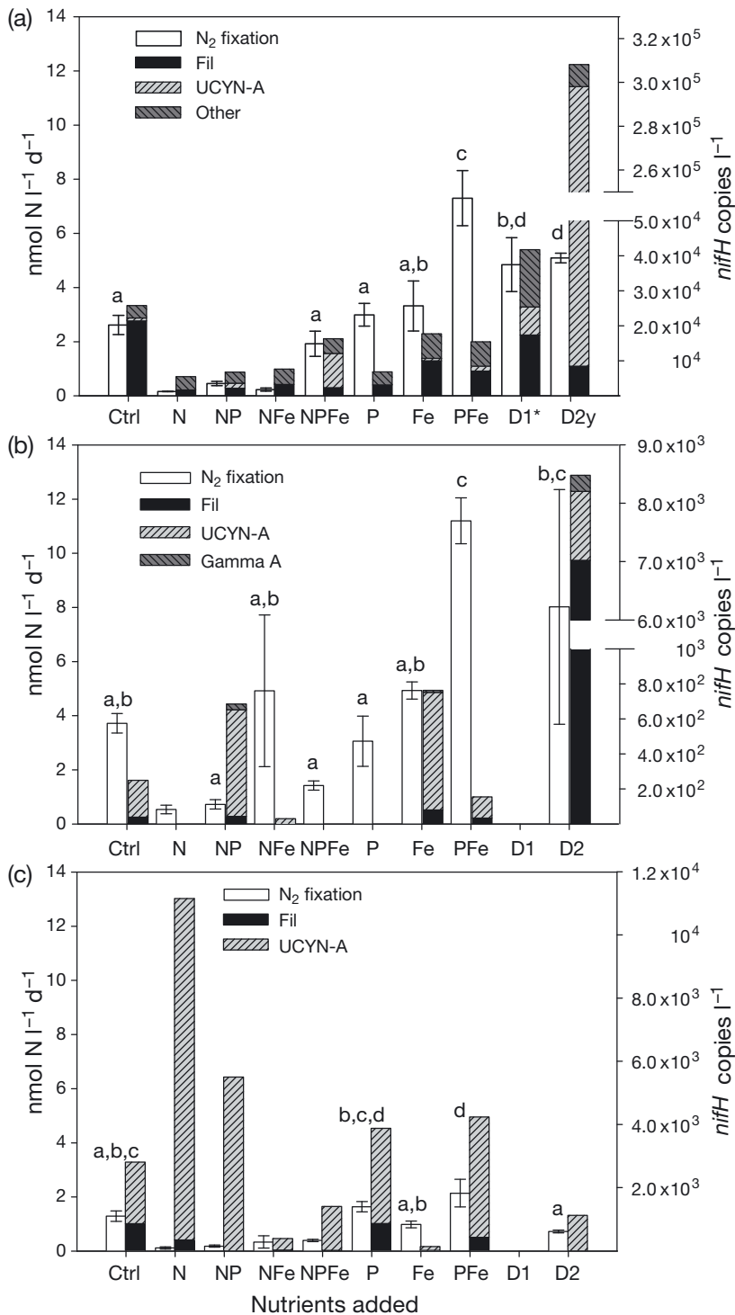
Fig. 2. Average ( \pm SE) N_2 fixation rates (nmol N l -1 d -1 ) and abundances of nifH phylotypes ( nifH copies l -1 ) detected in bioassay: (a) Expt A, (b) Expt B, (c) Expt C. Fixation rates for Expts A and B have been previously published (Mills et al. 2004) and have been re-plotted here. Letters identify mean N_2 fixation rates that are higher than or equal to the control (Ctrl) rate, and same letters denote means which are not statistically different from one another. Note that not all phylotypes are detectable in each experiment. *Only Expt A had the D1 (Dust) treatment. See 'Materials and methods' for detailed descriptions of treatments
