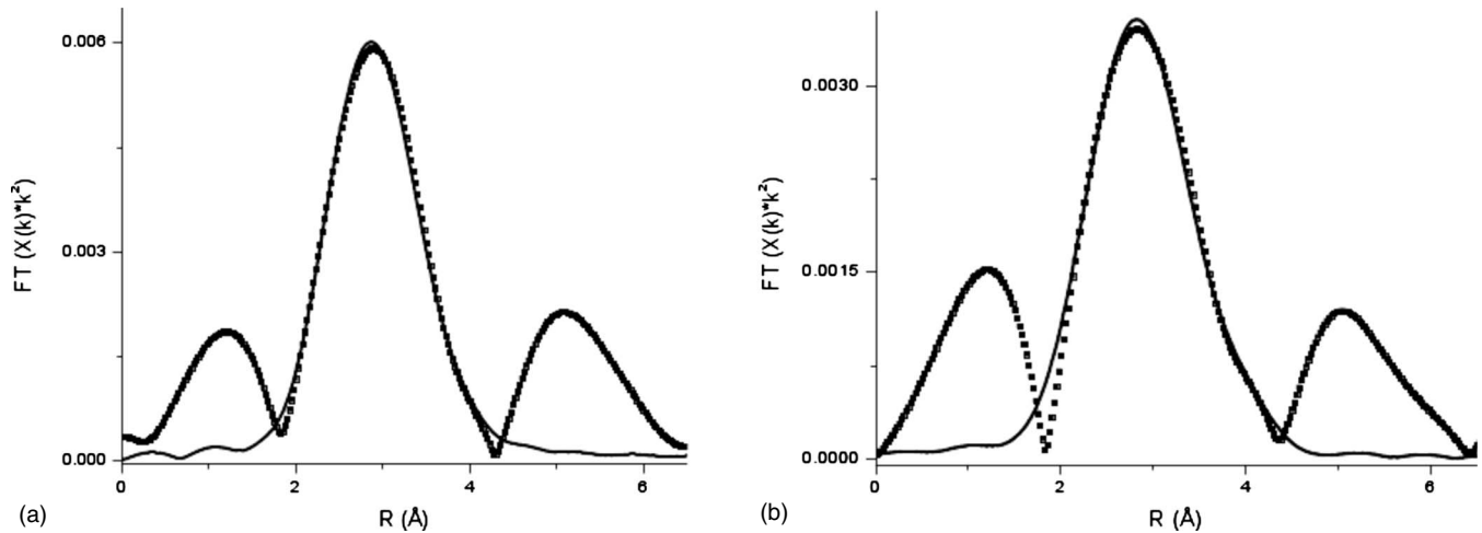
FIG. 3. EXAFS refinement. Experimental data (dots) and the fit (line) are presented for (a) \text{Na}_{21.5}\text{Si}_{136} and (b) \text{Na}_{14.1}\text{Si}_{136} .
