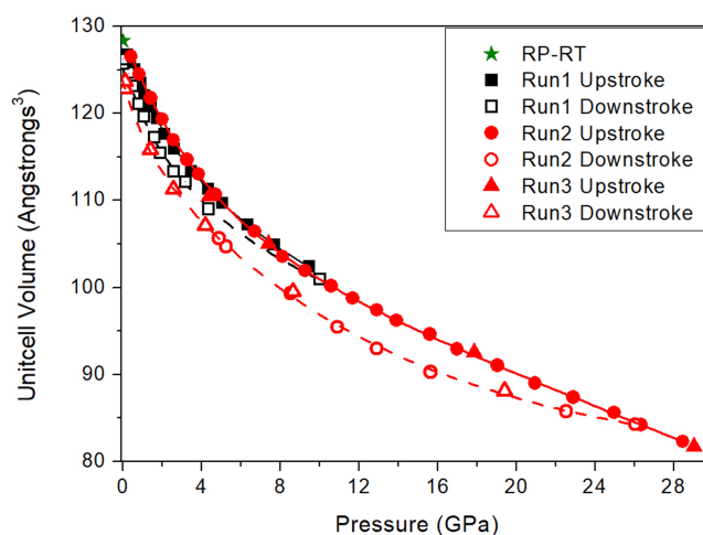
Fig. 3 \text{Au}_2\text{S} pressure-volume data from high-pressure XRD experiments. Run 1 (black symbols and line) used a 4:1 methanol:ethanol mixture as the pressure medium. Runs 2 and 3 (red symbols and line) used Ne as the pressure medium. During decompression there is a large hysteresis in the volume, which also depends on the maximum pressure reached and/or the pressure-transmitting medium. The green star symbol corresponds to the sample outside the DAC under ambient conditions.
