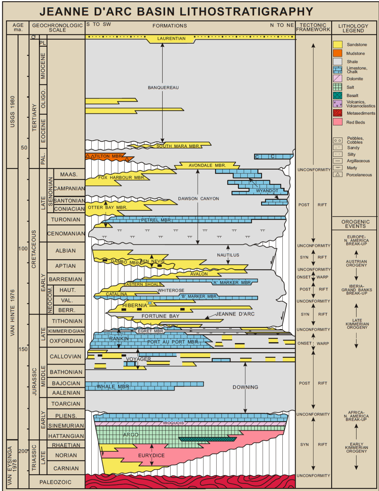
Figure 6. Stratigraphy of the Jeanne d'Arc Basin, offshore Newfoundland modified after Cohen, 2013.
