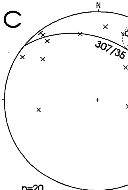
n=20 fabrics around nose Delaney's Brook Anticline
