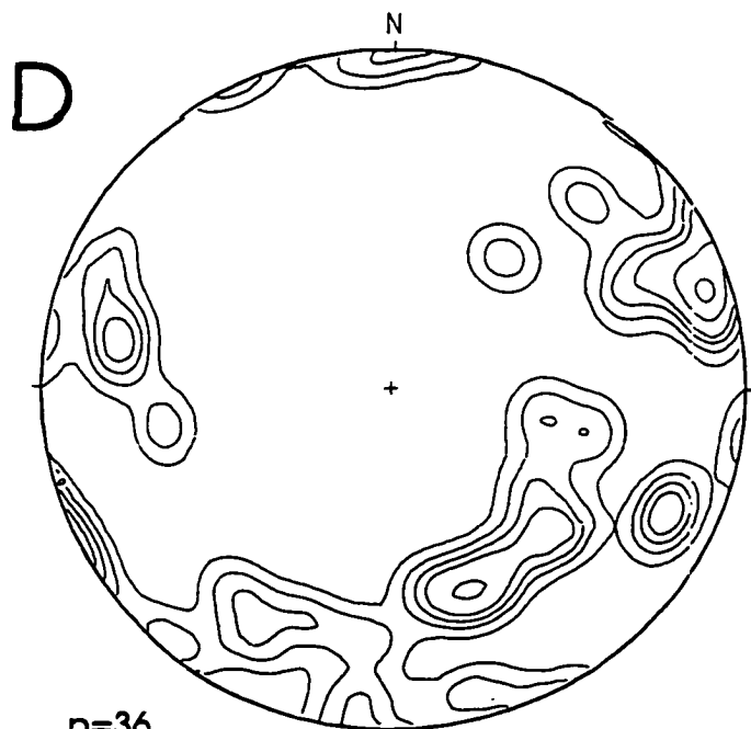
n=36 contours: 1,2,3,4,5% gneissic foliation in Polletts Cove River gneiss west of High Capes shear
