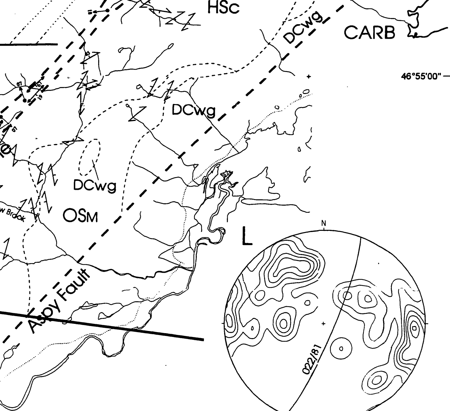
n=62 contours: 0.5, 1.5, 2.5, 3.5, 4.5, 5.5% layering and gneissic foliation in charnockite
