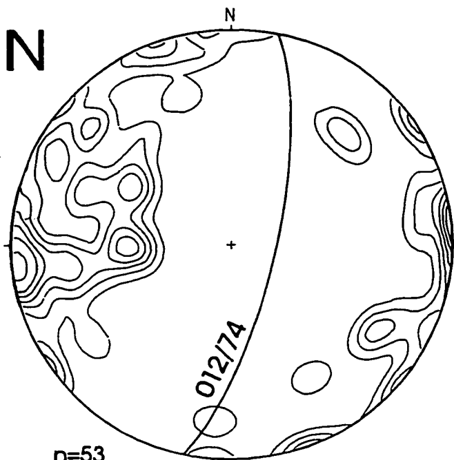
n=53 contours: 1,2,3,4,5% gneissic foliation in Otter Brook gneiss
