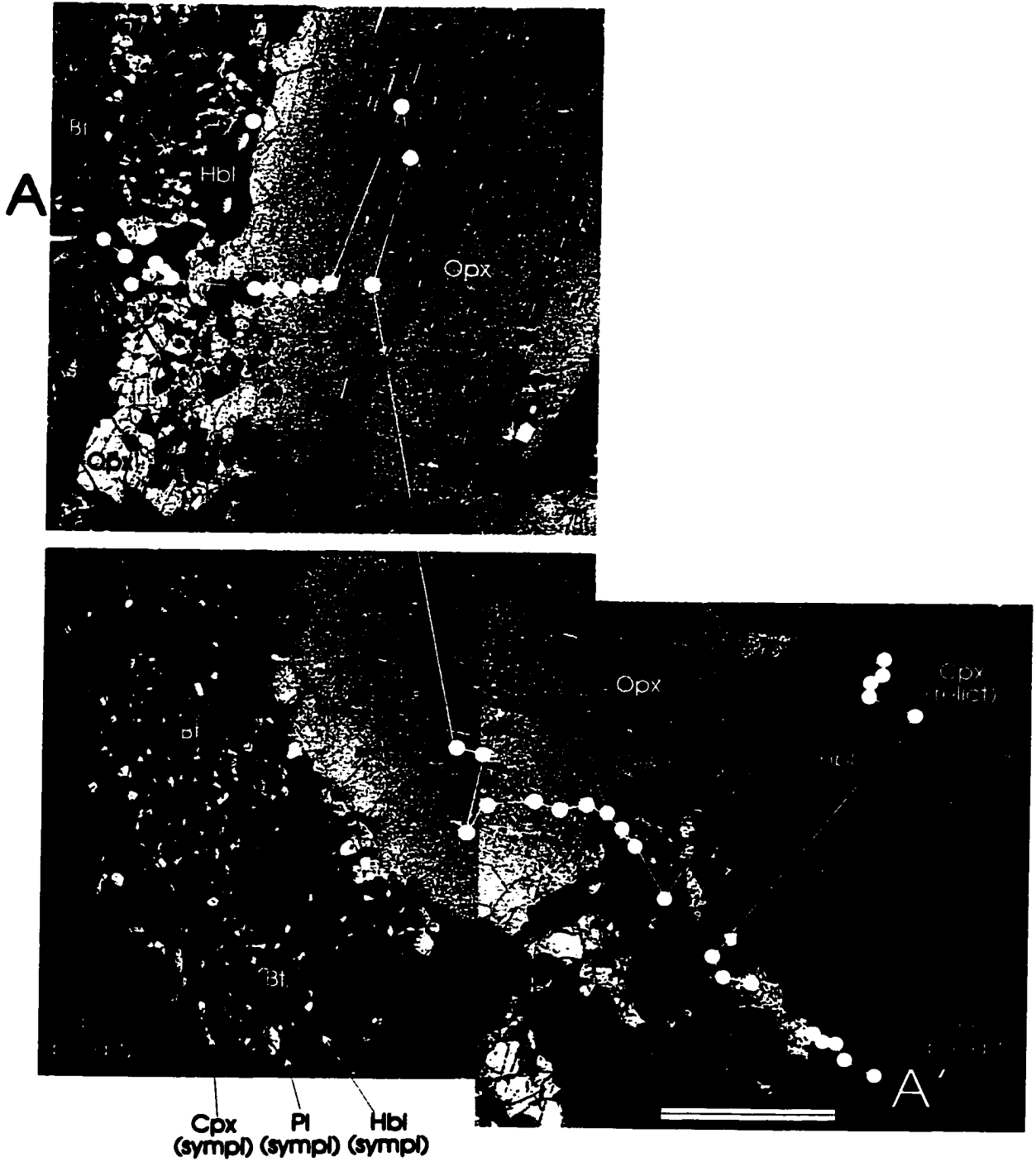
Figure 5.3 - BSE image mosaic of orthopyroxene auge in anorthosite sample BVM91-584 (pictured in Figure 5.2) from the Red River Anorthosite Suite. Microprobe traverse A-A' is shown and corresponds to the selected compositional parameters in Figure 5.4. Scale bar = 1 mm
