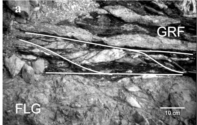
5-11: Systematic shear patterns and foliation in localized semi-brittle deformation zones, Brookville Rock. (a) Outcrop structures GRF- Greville River Formation; FLG - Fountain Lake Group. (b) Thin Section, Greville River Formation. Calcite-quartz fragments in phyllonitic matrix.
