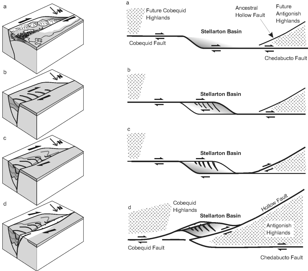
Fig. 4-3: Interpretive diagrams showing evolution of Stellarton Basin. Left: Development of an asymmetric pull-apart basin subsequently subjected to transpression. Right: Possible regional location of Stellarton Basin during its development.
