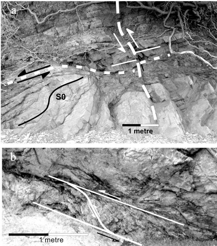
Fig. 5-3: Bedding-parallel thrusts typical of early transpressional deformation. (a) Low angle bedding-plane thrust faults in Parrsboro Formation are overprinted by high-angle reverse faults, both accommodating NNW-directed displacement. Photo facing N. (b) Thrusts within Windsor Group carbonate fault slice accommodate WNW-directed contraction. Greville Bay, internal zone. Photo facing E.
