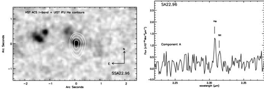
Figure 6. Left-hand panel: HST I_{814} -band image of SA 22.96 with the H\alpha emission from the UIST IFU observations overlaid as contours. Right-hand panel: collapsed spectra around the H\alpha emission from the western component (A) from the UIST IFU observations of SSA22.96. We identify A as the submm source at redshift z = 2.517 through identification of strong H\alpha and [\text{N II}] emission at the same redshift as derived from the rest-frame UV spectroscopy in Chapman et al. (2005). We note that there is tentative evidence for weak H\alpha emission from the structure \sim 1.5 arcsec to the east, suggesting it may be associated with the system.
