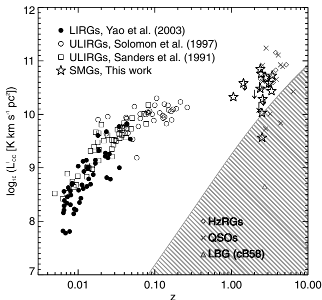
Figure 5. The relationship of \log_{10}(L'_{\text{CO}}) with redshift for the (ultra)luminous infrared galaxy (LIRG) samples of Sanders et al. (1991; SA91), Solomon et al. (1997; SO97) and Yao et al. (2003; Y03), and for the sample of high-redshift (sub)mm-selected sources presented in this paper. The CO luminosities have been corrected for gravitational amplification where necessary. Also shown are the (lensing-corrected) CO luminosities for high-redshift radio galaxies (HzRGs), quasi-sellar objects (QSOs) and Lyman break galaxies (LBGs) listed in Table 4, with the exception of Q 0957+561 and MG 0414+0534, which have unknown gravitational magnification factors. The CO luminosities for the (U)LIRGs are all based on the CO(1–0) line, whereas the luminosities of the high-redshift sources are entirely derived from CO J = J + 1 \rightarrow J transitions with J + 1 \geq 2 (Table 4). Upper limits on the CO luminosities for the seven SMGs not detected in CO are represented by downward pointing arrows. The hashed area denotes the region where sources are precluded from detection as a result of an integrated CO(3–2) flux limit of I_{\text{CO}} = 0.3 \text{ Jy km s}^{-1} . Of our sample, only SMM J16359+6612 with its very large amplification factor ( \mu = 22 ) is detectable below this limit.
