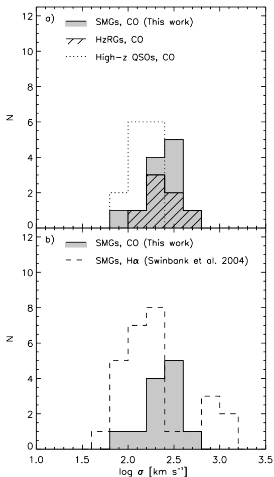
Figure 6. (a) Distribution of CO velocity dispersions for high-redshift quasi-sellar objects (QSOs) and high-redshift radio galaxies (HzRGs) from Table 2 and our sample of CO-detected submillimetre galaxies (SMGs). In the cases of the two high-redshift radio galaxies (HzRGs) 4C 60.07 and TN J0924–2201, we have adopted FWHM linewidths of 1000 and 325 \text{ km s}^{-1} , respectively. In (b), we compare with the measurements of the linewidths of the \text{H}\alpha line from near-infrared spectroscopy of a large sample of SMGs (Swinbank et al. 2004).
