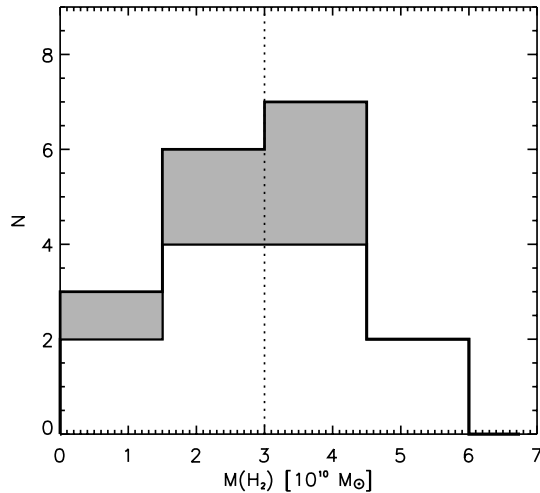
Figure 4. The distributions of molecular gas masses of the submillimetre galaxy (SMG) sample assuming a conversion factor of X_{\text{CO}} = 0.8(\text{K km s}^{-1} \text{pc}^2)^{-1} M_{\odot} and line ratios r_{32} = r_{43} = 1 . Non-detections are included as the shaded part of the histogram. The median gas mass of the sample, not including the non-detections, is \langle M(\text{H}_2) \rangle = (3.0 \pm 1.6) \times 10^{10} M_{\odot} (dotted vertical line).
