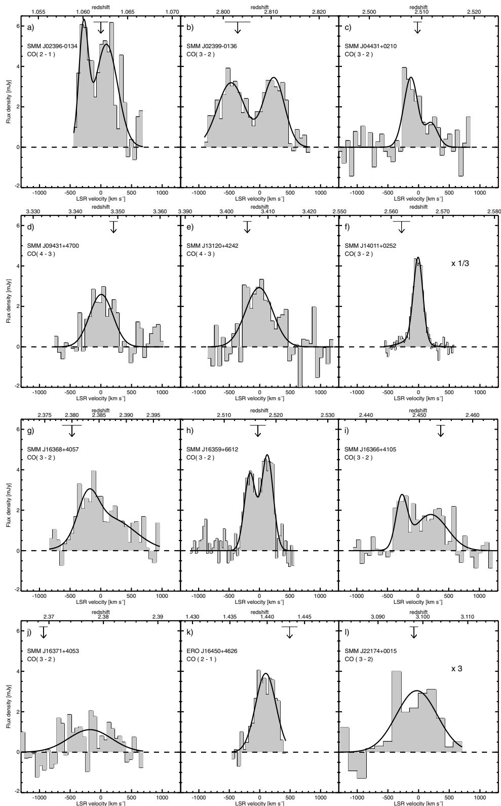
Figure 1. CO line profiles of the 12 submillimetre galaxies (SMGs) detected in CO to date. The profiles have been plotted on similar flux and velocity scales in order to facilitate an easy comparison between individual sources, to achieve this the spectra of SMM J14011+0252 and SMM J22174+0015 have been scaled by a factor of 1/3 and 3, respectively. The local standard of rest velocity scale is relative to the CO redshift. Optical redshifts are denoted by arrows and the horizontal bars on top of the arrows indicate the uncertainty of the redshifts. The redshifts derived from the CO lines are given in Table 2. The solid curves represent the best fits to the spectra using either single or double Gaussian profiles. The spectra shown in (c), (d) and (g) are taken from Neri et al. (2003); (h) is taken from Kneib et al. (2004), while (b), (f) and (k) are from Genzel et al. (2003), Downes & Solomon (2003) and Andreani et al. (2000), respectively. The spectra have been binned into 20 MHz bins, except for (f), (h) and (l) where the frequency binning is 7, 10 and 40 MHz, respectively.
