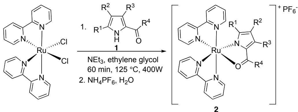
Scheme 1. Synthetic route to 2-formyl and 2-keto pyrrolide ruthenium(II) complexes.
