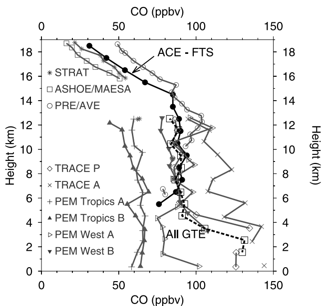
Figure 12. Tropical ( 20^{\circ}\text{S} – 20^{\circ}\text{N} ) CO climatologies from the ACE-FTS instrument and from various aircraft campaigns. The thick dashed line is an average over all four Pacific Exploratory Experiment (PEM) campaigns and the two Transport and Atmospheric Chemistry (TRACE) campaigns.
