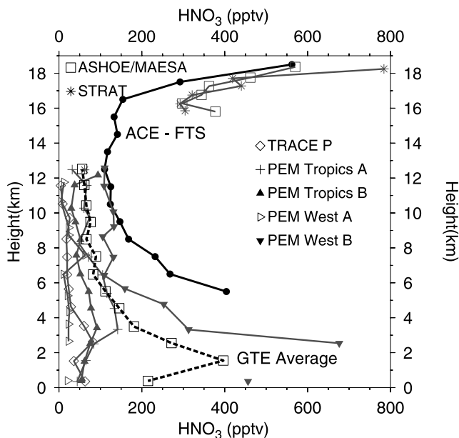
Figure 14. An intercomparison of tropical ( 20^{\circ}\text{S} – 20^{\circ}\text{N} ) \text{HNO}_3 climatologies from ACE-FTS and various aircraft campaigns. The thick dashed line is an average of the \text{HNO}_3 climatologies from the four Pacific Exploratory Mission (PEM) experiments and the Transport and Atmospheric Chemistry in the Pacific (TRACE-P) experiment. The ASHOE/MAESA and STRAT plots refer to inferred rather than directly measured nitric acid (i.e., \text{HNO}_3^* = \text{NO}_y - \text{NO}_x ).
