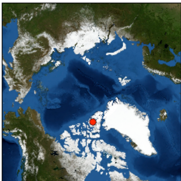
Fig. 1. Polar map of the Arctic. The location of Eureka ( 80^{\circ}\text{N} , 86^{\circ}\text{W} ) is marked with a red dot.
