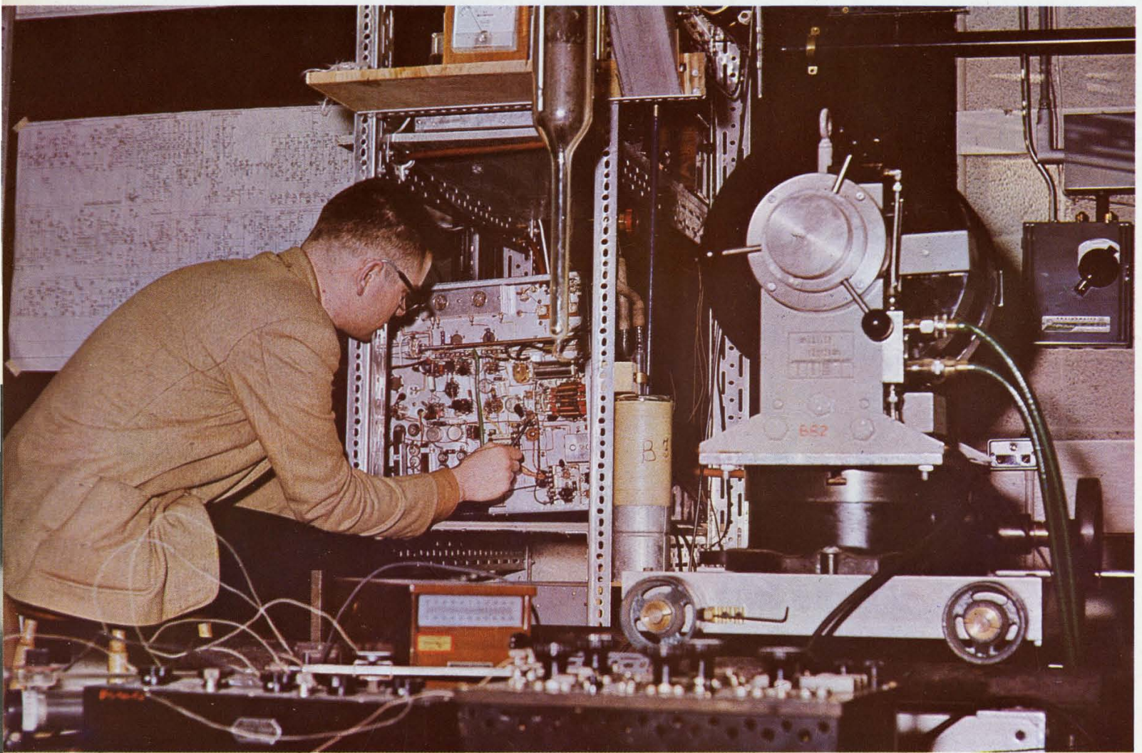
A Research Experiment in Physics
