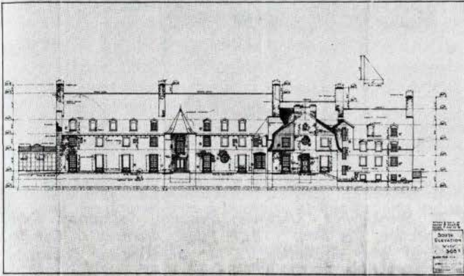
Fetherstonhaugh & Durnford. "South elevation Arvida Inn, Aluminum Co. of Canada Ltd., Arvida, PQ." 1939. Public Archives of Canada, National Map Collection, H. L. Fetherstonhaugh Collection, 81203/1, project 835, item 6. C 95384.
