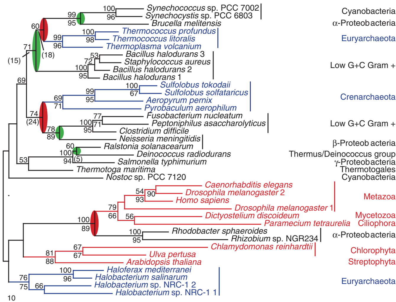
Figure 2 Maximum likelihood tree of GDH-2 The phylogenetic tree is based on 305 unambiguously aligned amino acid positions. The \Gamma shape parameter, \alpha , and the fraction of invariable sites, P_{inv} , were estimated to 1.10 and 0.08, respectively. The tree is arbitrarily rooted. Labeling as in Figure 1 with the addition that Archaea are labeled in blue.
