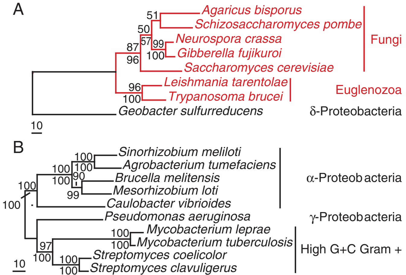
Figure 3 Maximum likelihood trees of GDH-3 and GDH-4 (A) The phylogenetic tree is based on 457 unambiguously aligned amino acid positions of GDH-3. The \Gamma shape parameter, \alpha , and the fraction of invariable sites, P_{inv} , were estimated to 1.07 and 0.06, respectively. (B) The phylogenetic tree is based on 1141 unambiguously aligned amino acid positions of GDH-4. The \Gamma shape parameter, \alpha , and the fraction of invariable sites, P_{inv} , were estimated to 1.14 and 0.14, respectively. The trees are arbitrarily rooted. Labeling as in Figure 1.
