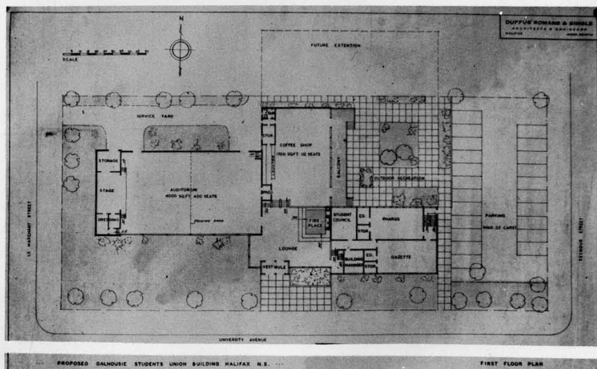
Floor plan of the proposed Dalhousie Student Union Building.
