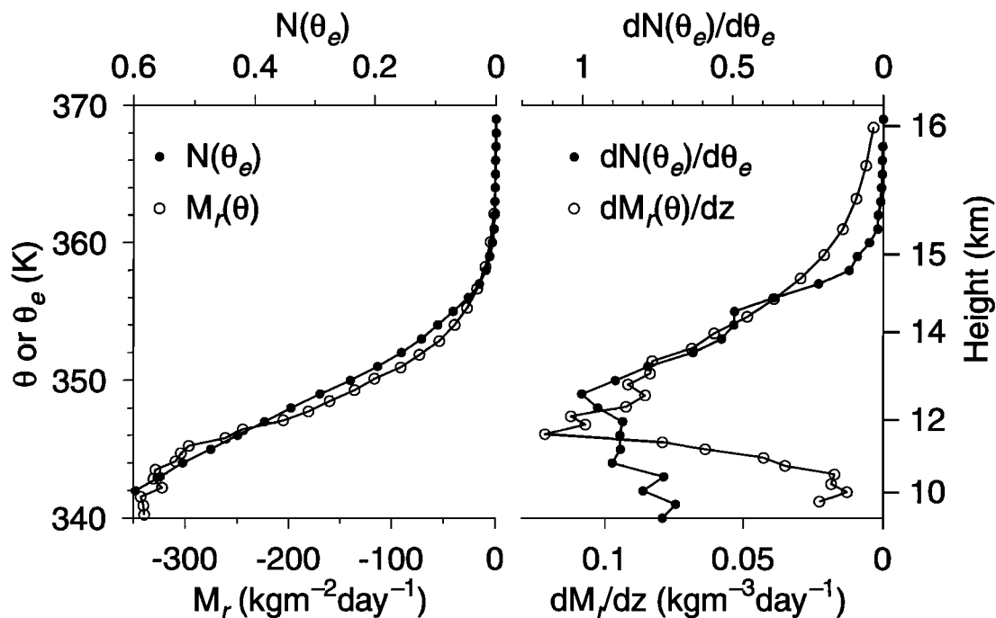
Figure 2. (left) The curve with open circles is the clear sky vertical mass flux M_r(\theta) as obtained from (1) in the text. The curve with solid circles is N(\theta_e) from Figure 1, but with the axes interchanged. (right) The curve with open circles is dM_r(\theta)/dz . The curve with solid circles is dN(\theta_e)/d\theta , also from Figure 1 with the axes interchanged.
